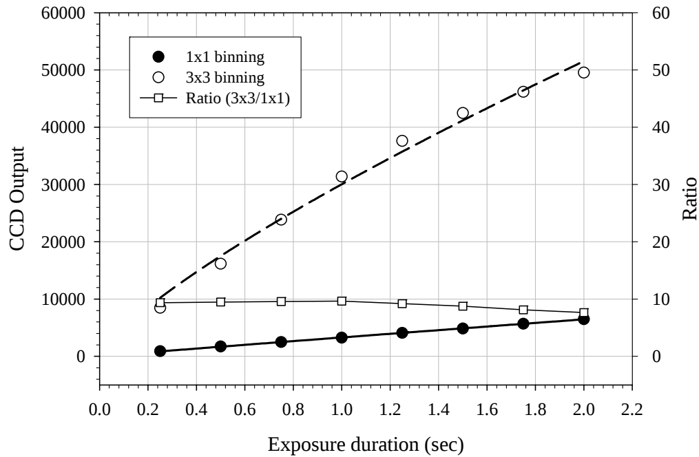
Figure 10 Effect of CCD binning and exposure duration on CCD output.
