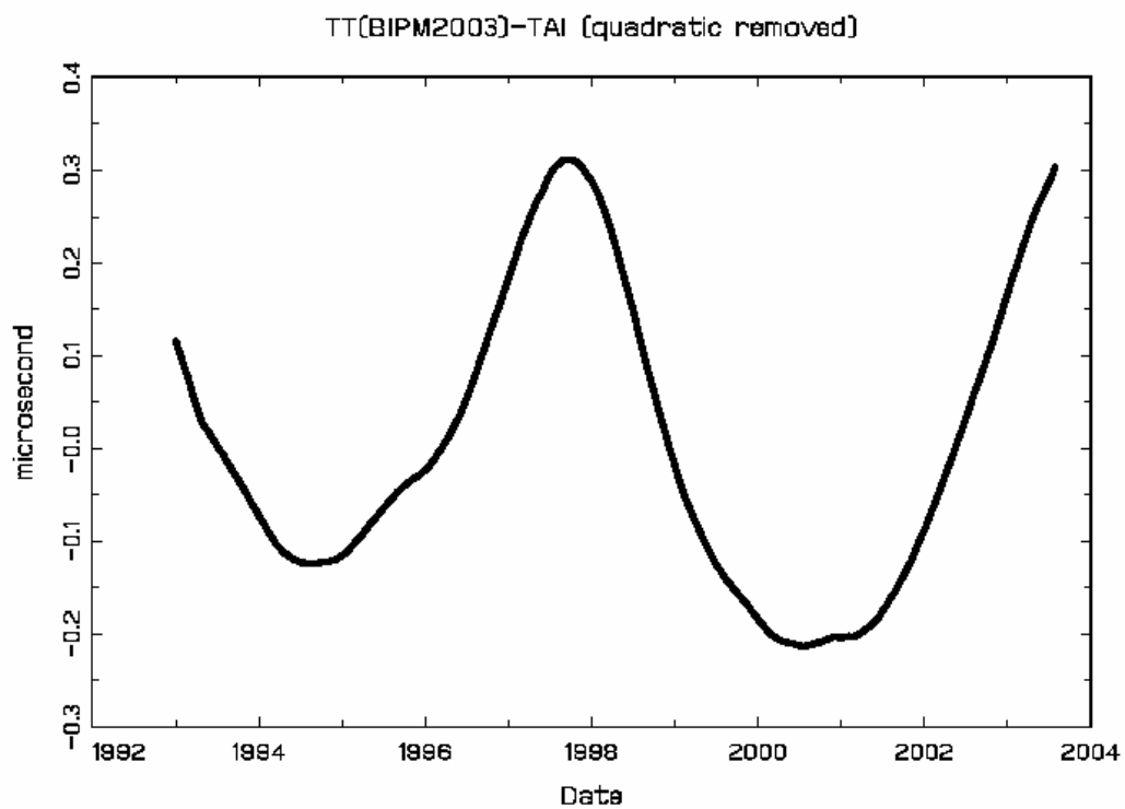
Figure 2. Effect on pulsar analysis of using TT (BIPM2003) or TAI as a reference.
