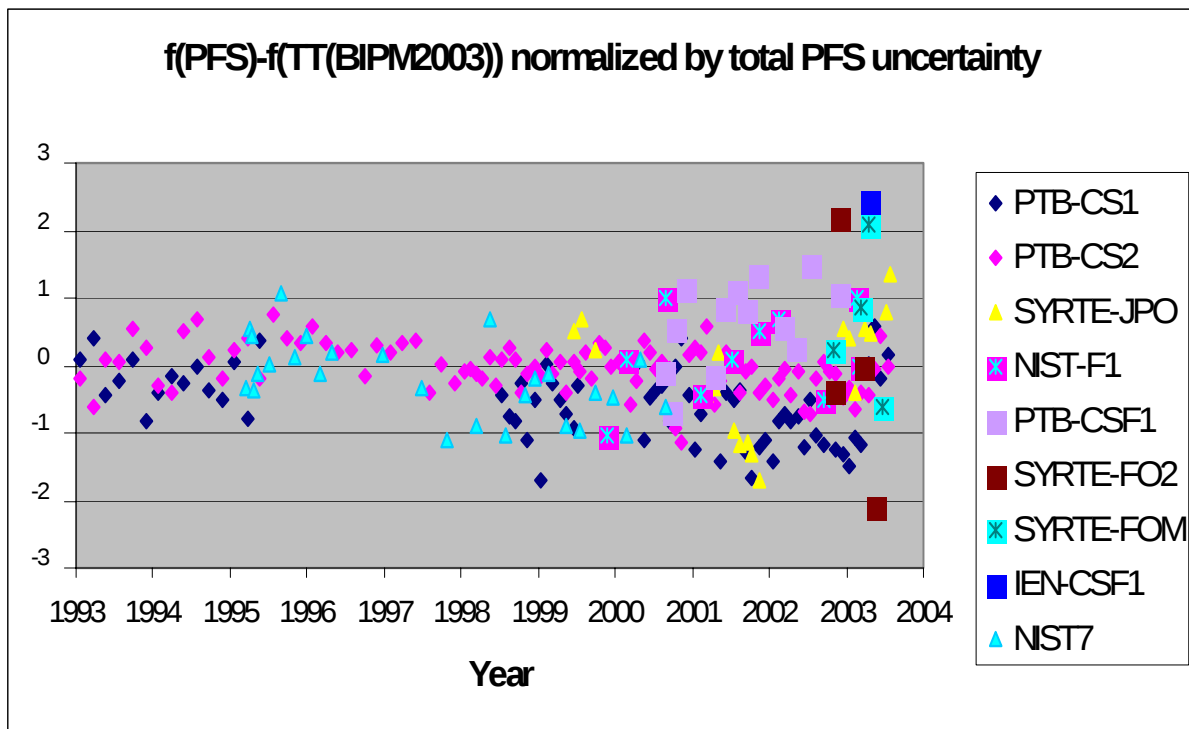
Figure 4. f(\text{PFS} - \text{TT}(\text{BIPM2003})) normalized: data of Figure 3 divided by their total standard uncertainty.
