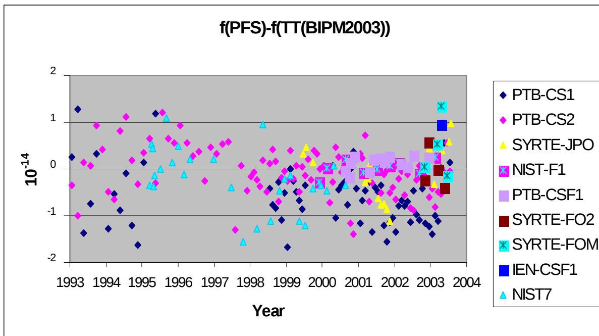
Figure 3. f(\text{PFS} - \text{TT}(\text{BIPM2003})) for all measurement of nine primary frequency standards over 1993-2003.
