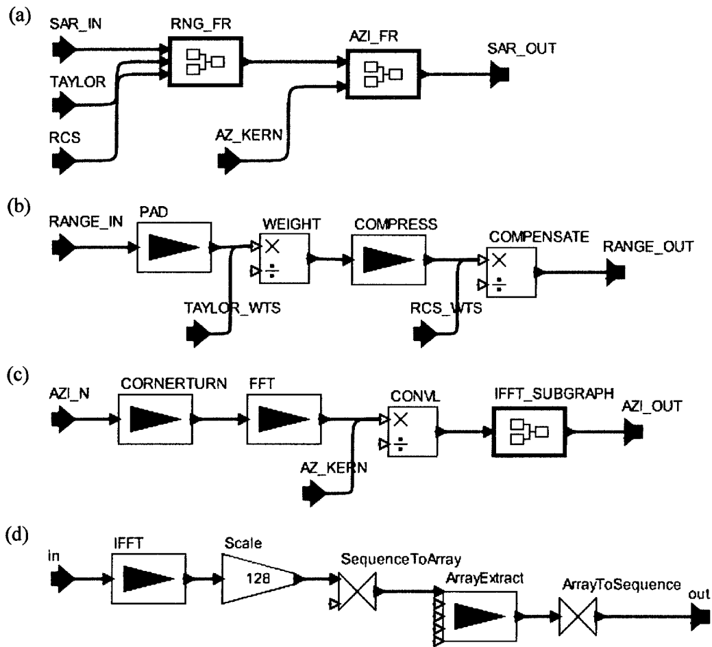
Figure 19. The SAR benchmark application in Ptolemy. (a) SAR_FR graph. (b) RNG_FR graph. (c) AZI_FR graph. (d) IFFT_SUBGRAPH graph
