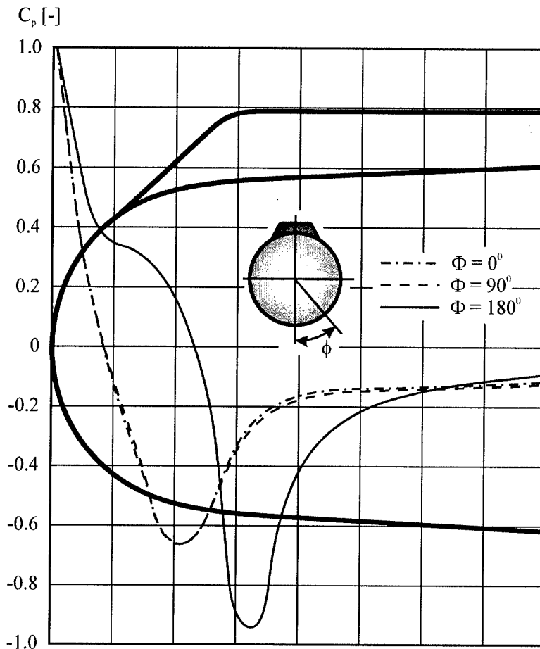
Figure 31. Pressure distributions on a forebody with an integrated hydrophone [33].
