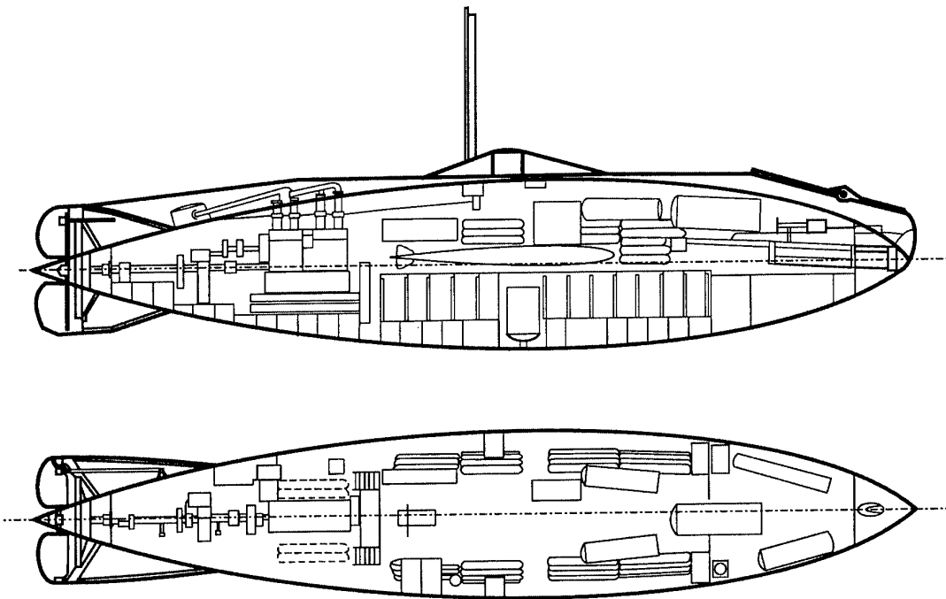
Figure 1. Profile of Holland [7, p.11]
