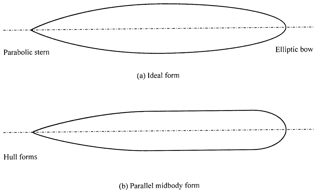
Figure 12. Hull forms
