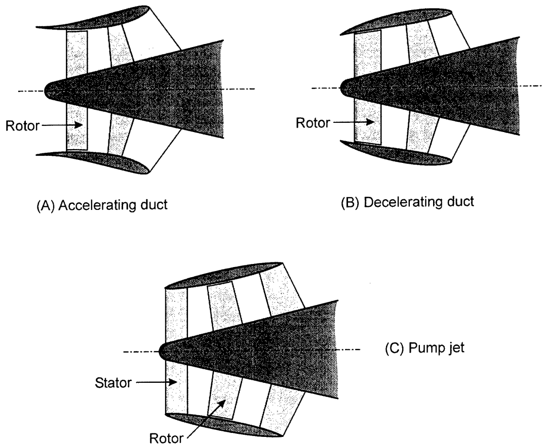
Figure 34. Types of ducted propulsors
