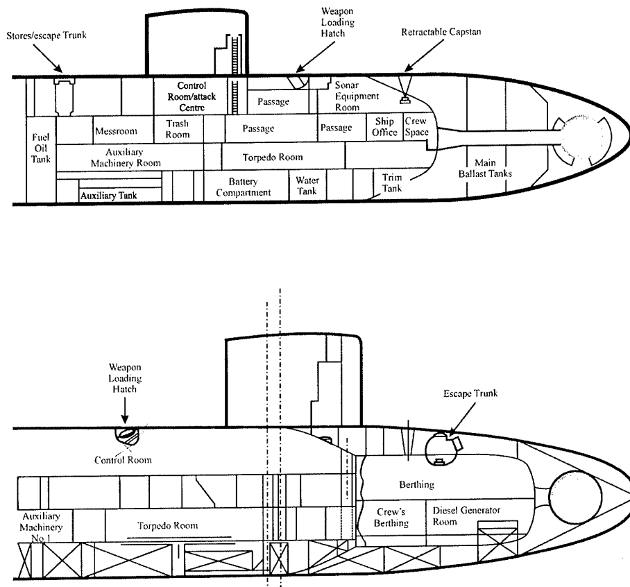
Figure 30. Bow sonars on US Los Angeles and US Sturgeon showing nose-shape and torpedo tubes.
