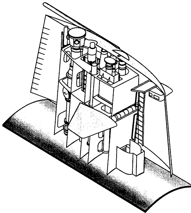
Figure 27. Shaft connecting sail mounted hydroplanes [46]
