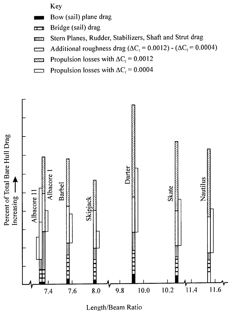
Comparative appendage resistance, roughness drag, and propulsion losses for submarine forms of 100,000 cubic foot volume.
