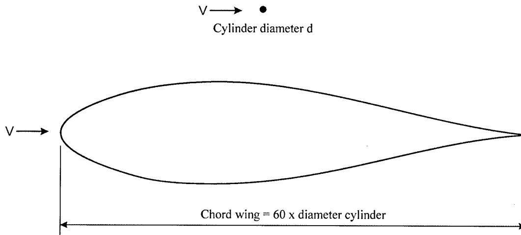
Figure 21. Drag of cylinder equals drag of streamlined shape
