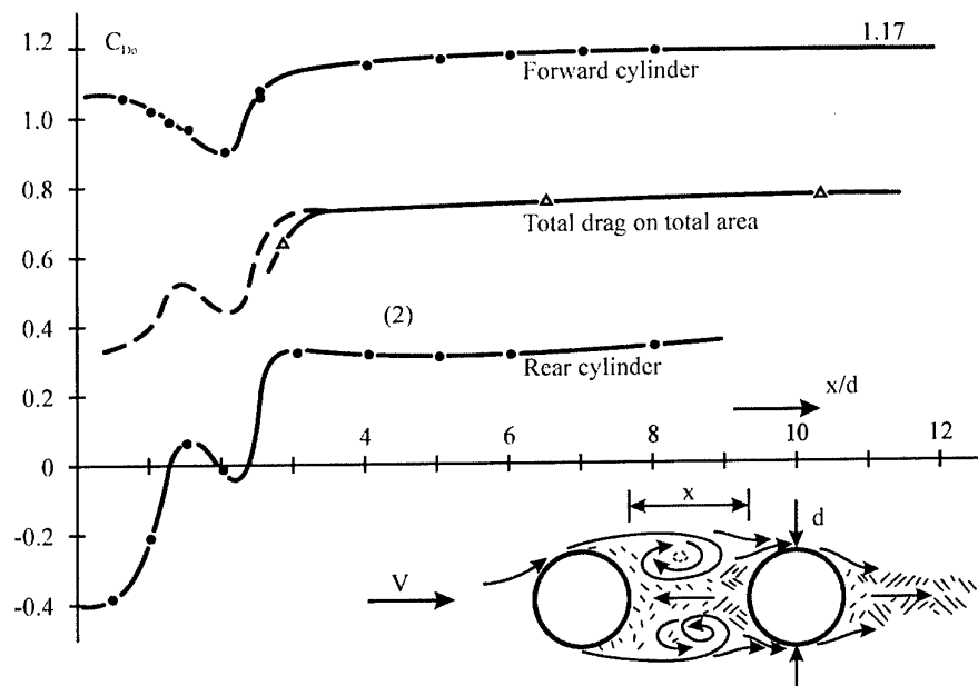
Figure 24. Drag coefficients of two circular cylinders, one placed behind the other.
