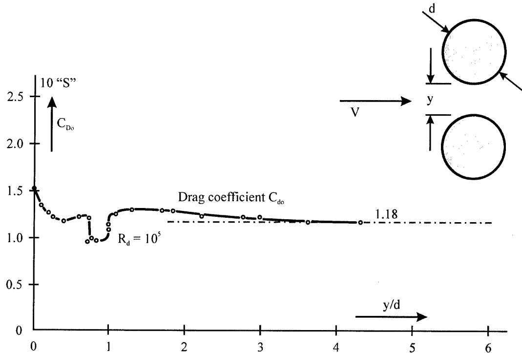
Drag (2,a) of a pair of circular cylinders placed side by side
