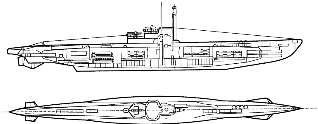
Figure 4. Type VII C. Typical of a World War II German Submarine [11]
