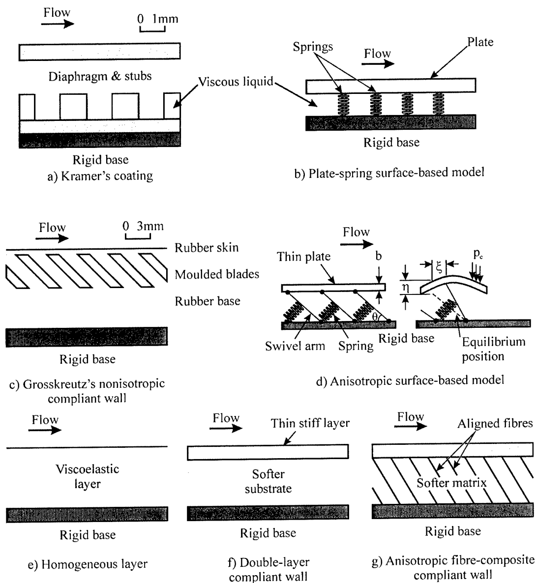
Figure 35. Volume-based and surface-based models of compliant coatings [43].
