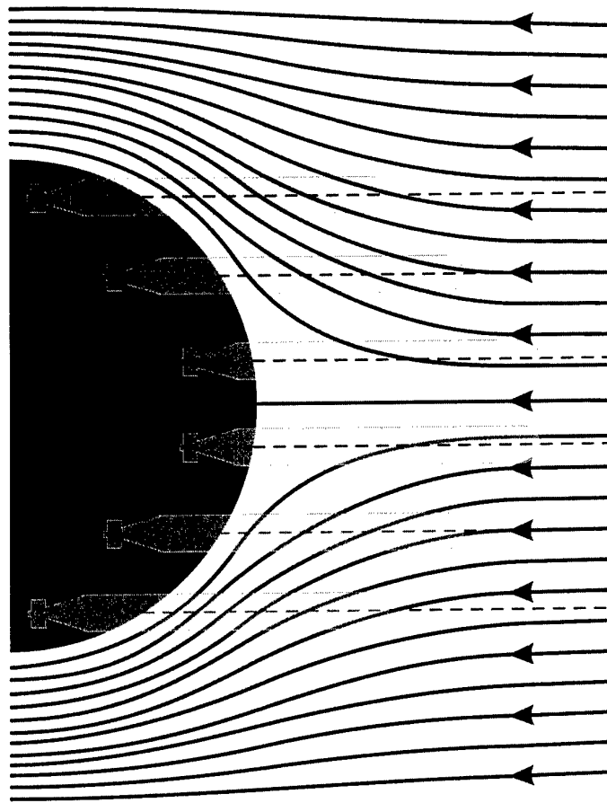
Figure 32. Bow streamlines on a hemisphere. Dashed lines of torpedo tubes.
