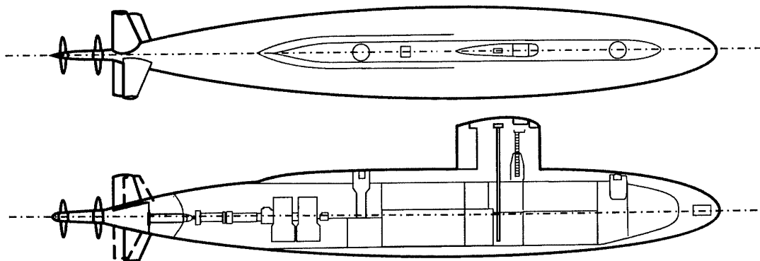
Figure 7. Albacore (4 th Modification) [4]
