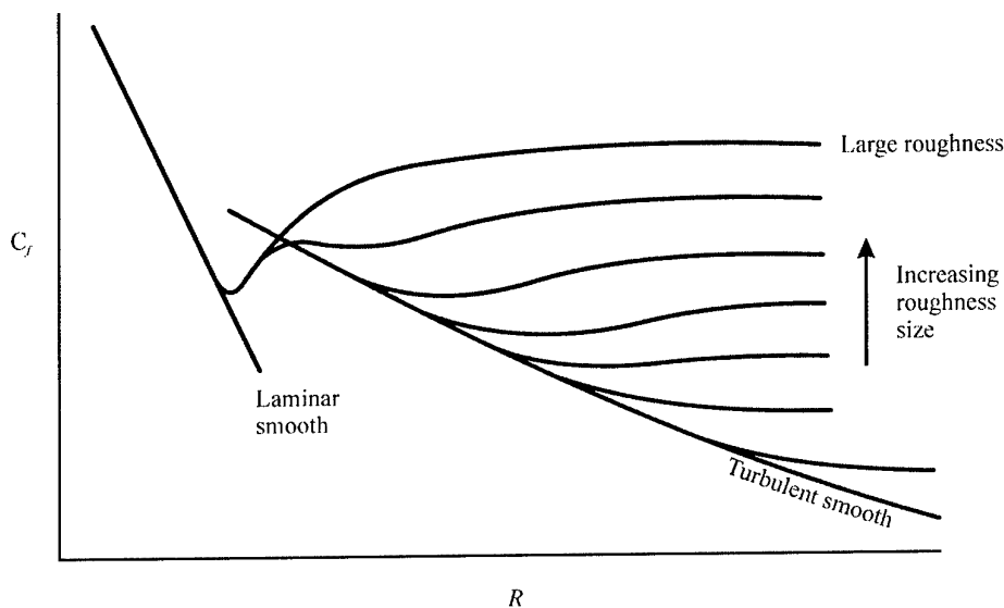
Figure 18. Sketch illustrating variation of friction drag of a plate at zero incidence with roughness height.
