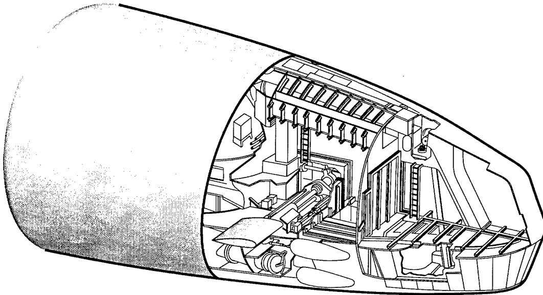
Figure 29. Cutaway drawing HMS Swiftsure [7]
