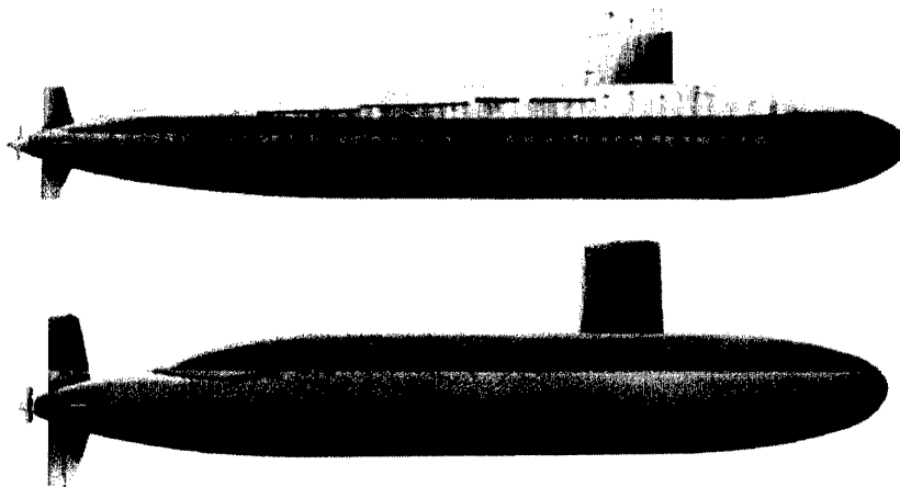
Figure 14. Profiles of Japanese submarines Yuushio (1979) and Harushio (1989) respectively [6].
