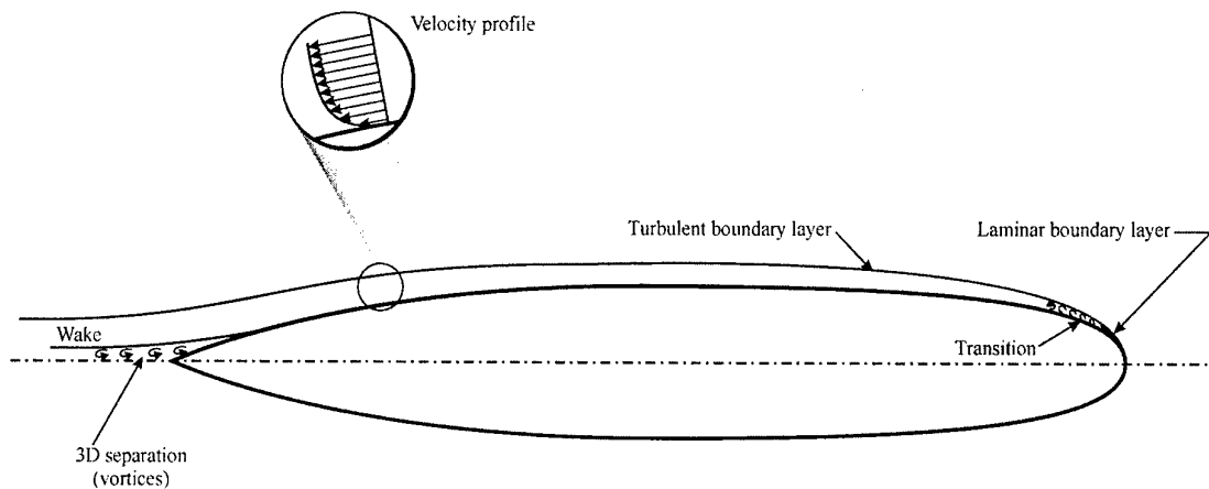
Figure 16. Flow around a submarine
