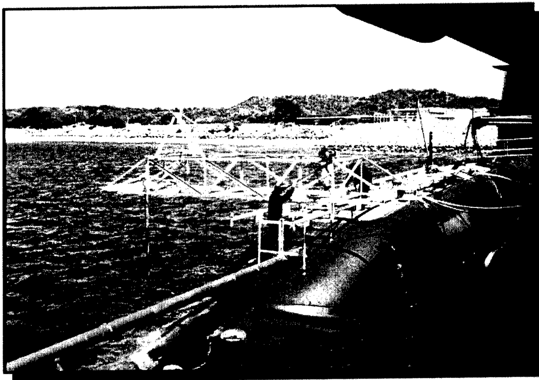
Figure 26. Fixed tube for towed array
