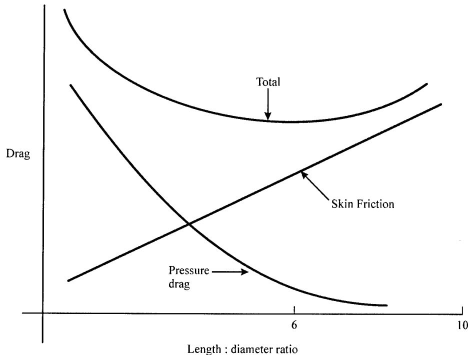
Figure 11. Drag components for constant volume form [1, p.105]
