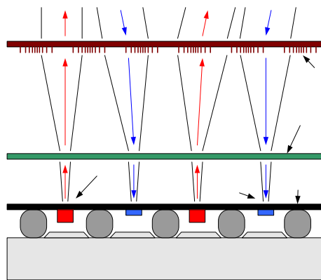
Figure 2. Integration configuration for optoelectronic substrate modules
