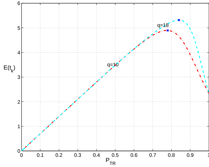
Figure 6.2 Scenario 2: Expected number of TK for two sensors, w = 10 , \lambda_{FT} = 20 , \lambda_T = 10 , P_k = 0.7 , x = 1
