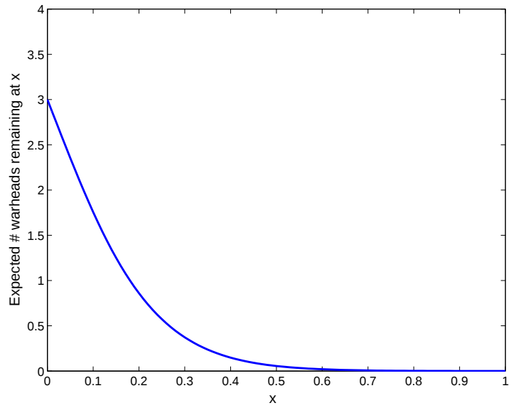
Figure 4.2 Expected number of warheads remaining at x : \lambda_{AT} = 3 , \lambda_{FT} = 10 , w = 3
