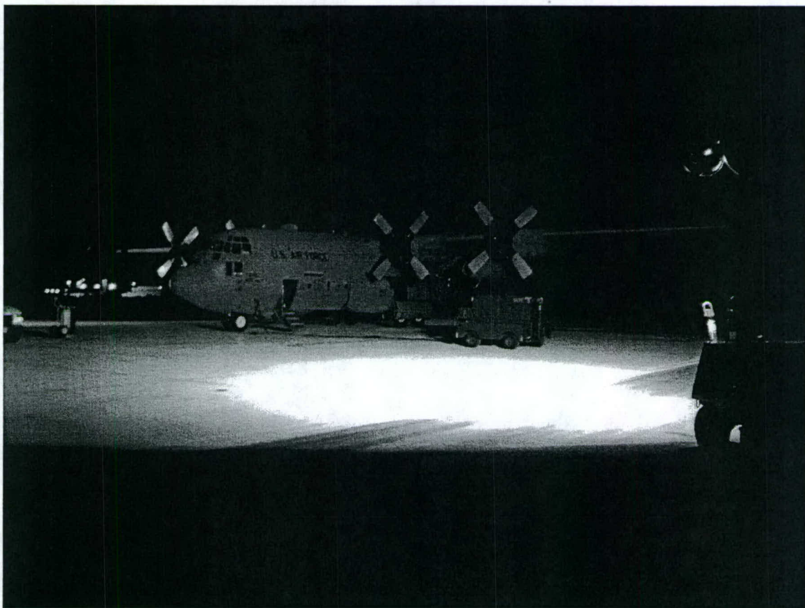
Early morning picture of C-130H on the static thrust stand at Edwards AFB.
