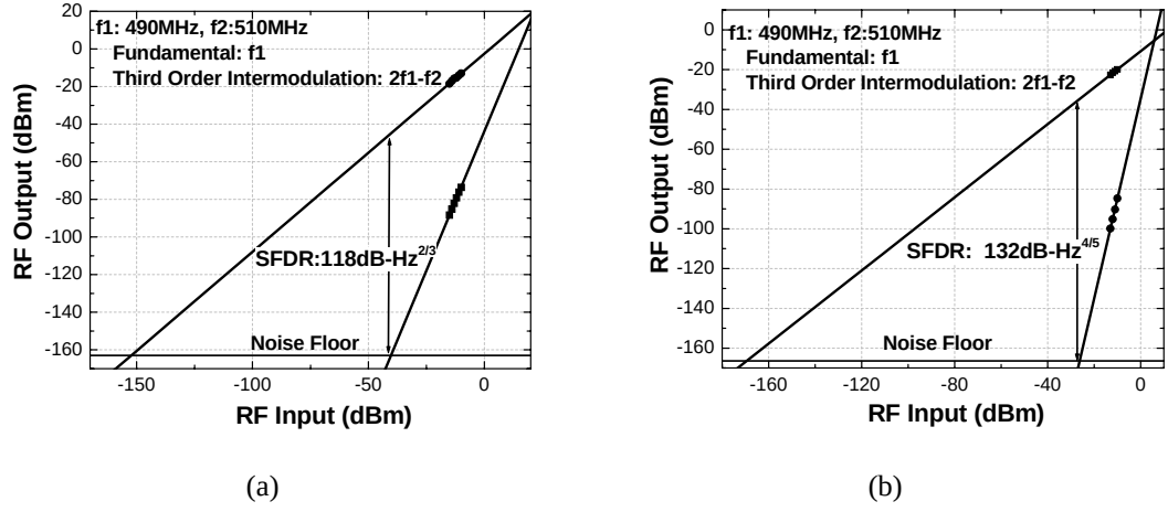
Fig. 4 (a) Measured fundamental and 3 rd order intermodulation distortion signals at the second order null bias point, (b) measured fundamental and 3 rd order intermodulation distortion (5 th order nonlinearity dominated) at the 3 rd order null bias point.
