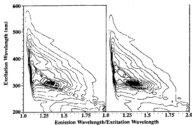
Figure 7: (A) Fluorescence spectrum of dry CaDPA without UV exposure on filter paper. (B) Fluorescence spectrum of UV exposed dry CaDPA crystals on filter paper. The excitation was stepped every 10 nm from 200 to 600 nm. The intensity is equally divided by 15 contour lines. The greatest intensity is dark and the least intensity is white. The maximum intensity on (B) is 1.5 times larger than the maximum intensity on (A).
