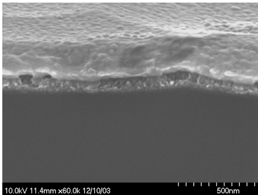
Figure 4.10. Cross-sectional SEM image of an unannealed contact composed of 50 Å Ti, 1500 Å Ni, and 500 Å Au. The substrate is crystalline SiC.
