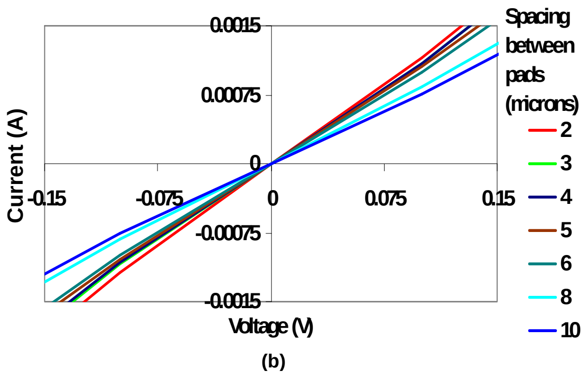
Figure 4.13. I/V data collected from a row of contact pads composed of 50 Å Ti, 1500 Å Ni, and 500 Å Au annealed at 900 °C for 10 min. The substrate is crystalline SiC. (a) is shown in full scale, while (b) has the current scale enlarged to show detail.
