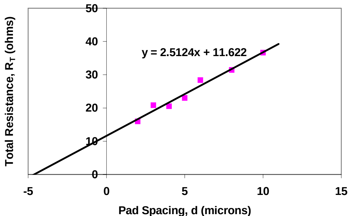
Figure 4.14. TLM data collected from a row of contact pads composed of 50 Å Ti, 1500 Å Ni, and 500 Å Au annealed at 900 °C for 10 min. The substrate is crystalline SiC. Analysis of the data according to Eqs. 4.2-4.5 yields a specific contact resistance of 1.3 \times 10^{-5} \Omega \text{ cm}^2 for these contacts.
