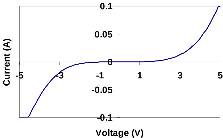
Figure 4.9. I/V curve of an unannealed 150 nm thick nickel contact to crystalline SiC, showing the expected Schottky character.
