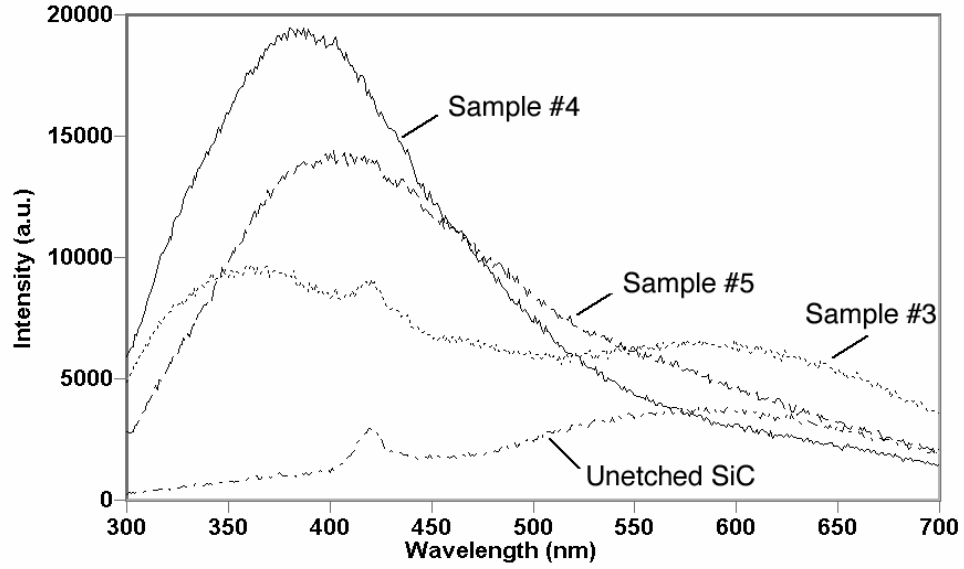
Figure 3.3. Cathodoluminescence spectra of unetched 6H-SiC and three different pieces of PSiC prepared from n-type 6H-SiC by anodic etching for 40 min. Sample numbers correspond to the notation given in Table 2.1 of Chapter 2.
