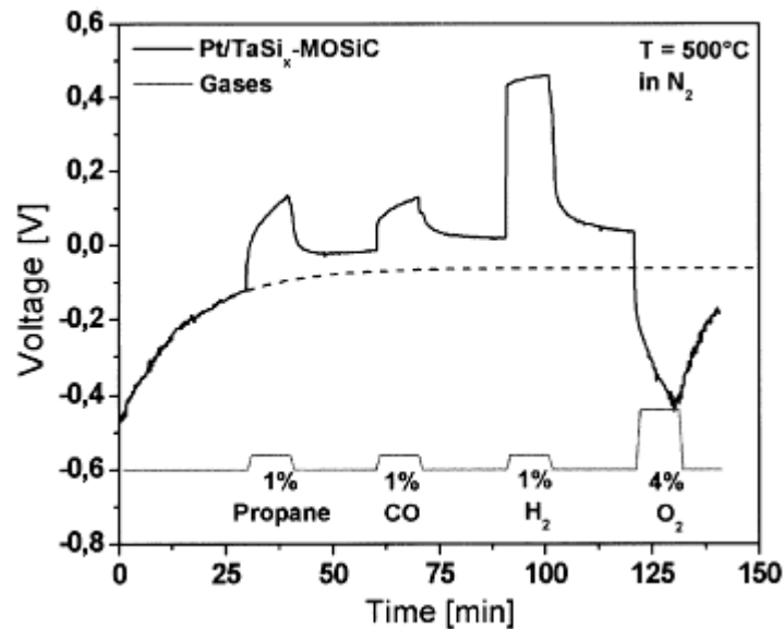
Figure 4.4. 46 Data showing drift in the baseline conditions for a Pt-TaSi-SiC Schottky diode sensor operating at 500 °C. The sensor drift is believed to be due to slow desorption of surface oxygen ions from the sensor during the exposure to the N 2 background atmosphere.
