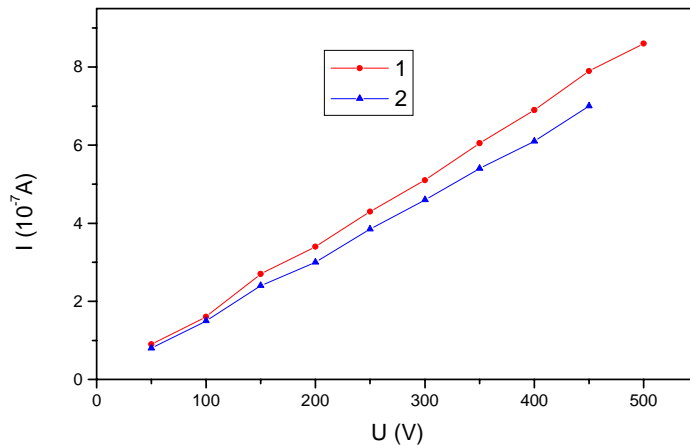
Fig.1. Current-voltage characteristics for the two structures metal-polymer-metal at T = 300 K. Curve 1 for molybdenum-polymer- molybdenum structure and curve 2 for aluminum-polymer-aluminum structure.
