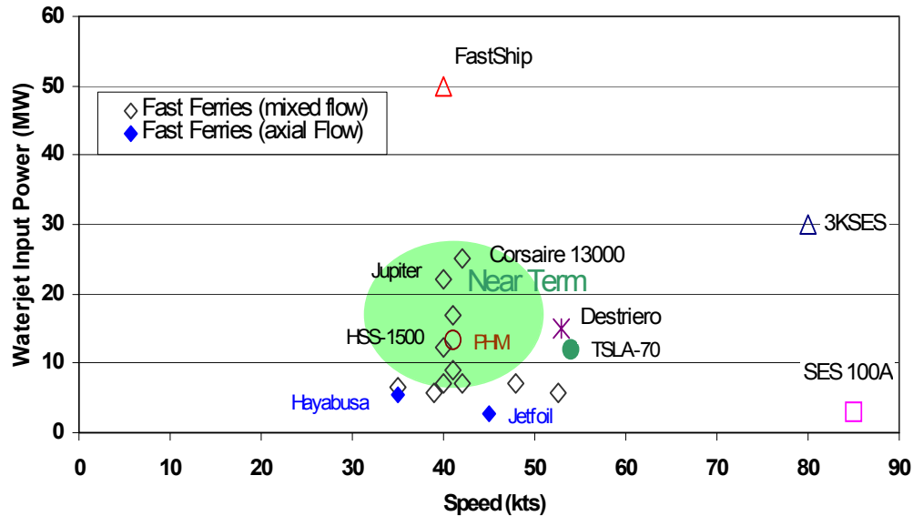
Figure 5.3.2-2: Waterjet Technology
