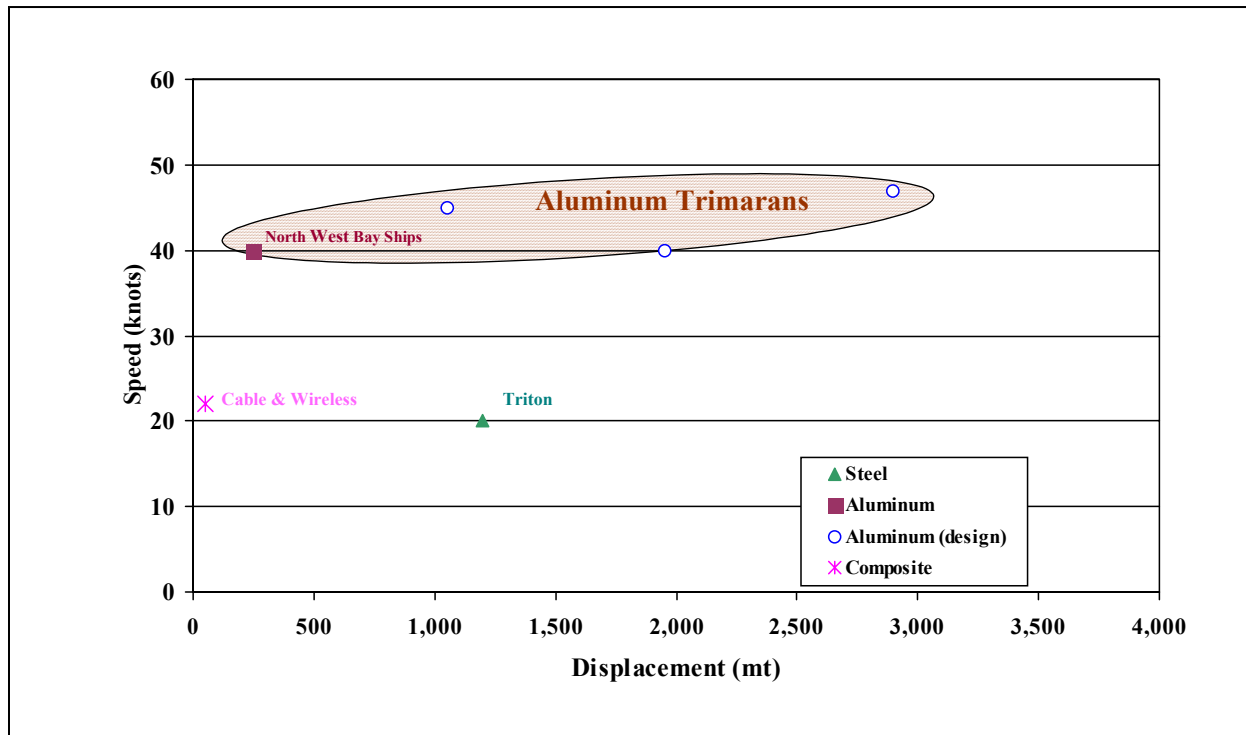
Figure 2.4.1-4: Trimaran Technology
