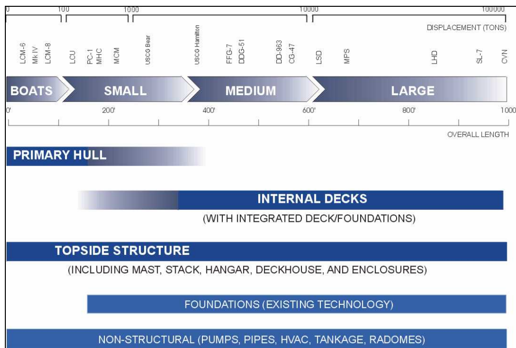
Figure 4.4.1-3: Composite Applications
