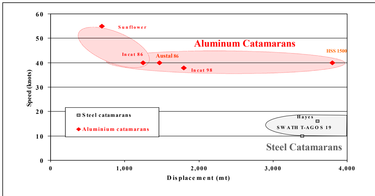
Figure 2.3.1-3: Catamaran Technology
