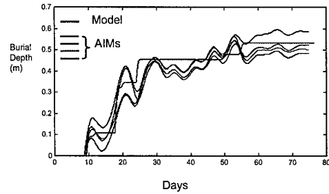
Fig. 23. Comparison of forecast for scour induced burial of cylindrical model to actual AIMs burial.
