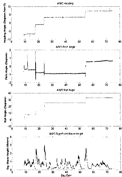
Fig. 14. Heading, Roll, Pitch and Significant Wave Height for AIM #3.
