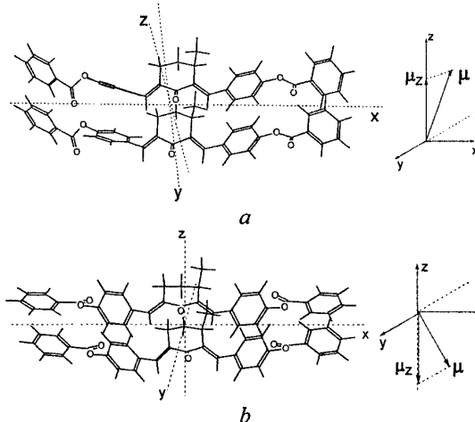
Fig. 4. Binary molecular ensembles of 1c with different polarity and energetics: A (a) and D (b) (see Table 3)
