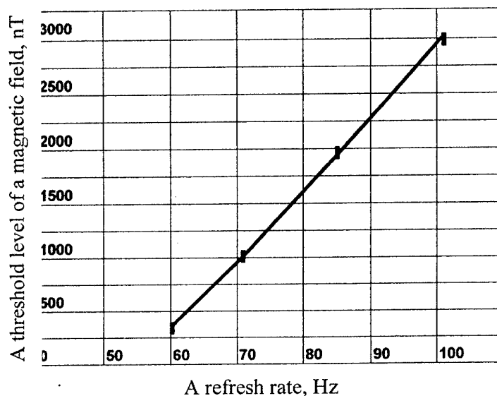
Figure 1. Dependence of a threshold level of a magnetic field on a refresh rate of an image for one from types of displays with a screen 17".
