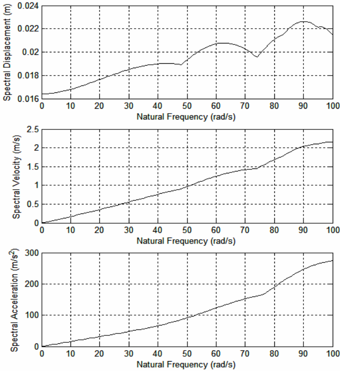
Figure 3. Shock-Response Spectra Using the Induced-Displacement Input of Table 1, for damping ratio 0.1.
