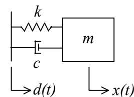
Figure 1. Hypothetical SDOF MSD system, for SRS determination
