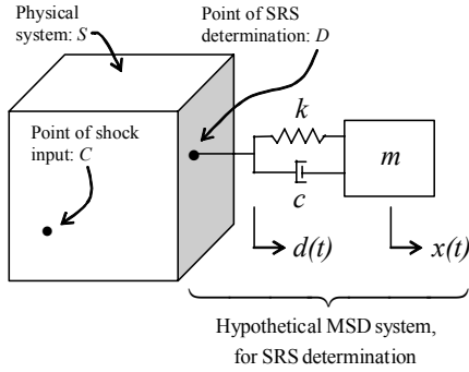
Figure 2. Shock-loaded system S , with (hypothetical) attached MSD system for SRS determination
