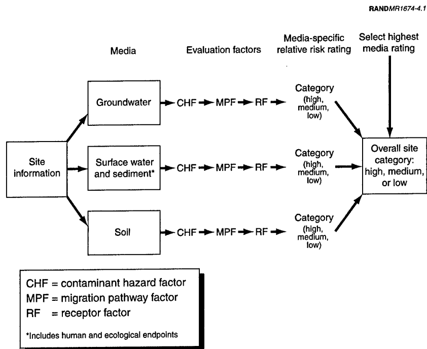
Figure 4.1—Flow Diagram Showing Inputs to and Output from the Relative Risk Site Evaluation
