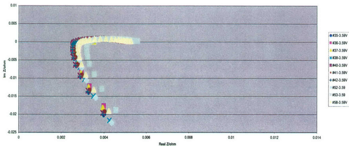
Figure 8. Nyquist plots for group M047xx18 after acceptance testing.
