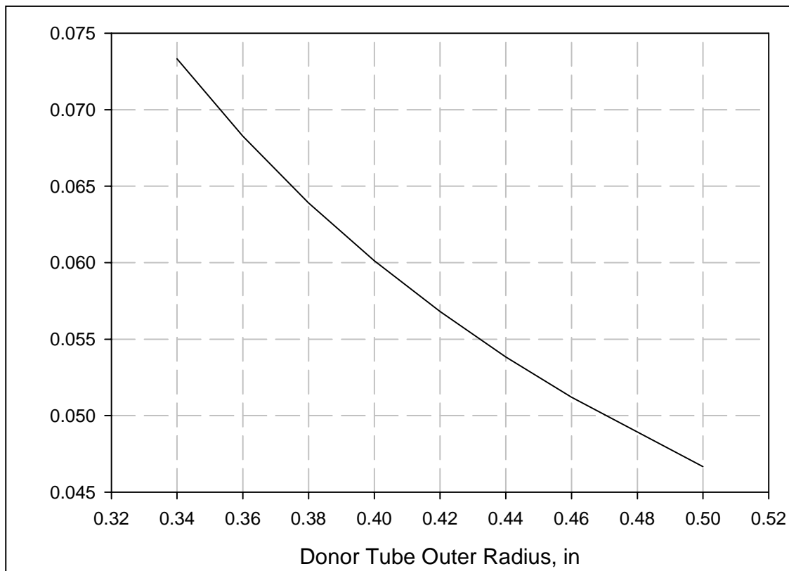
Figure 1. Donor tube wall thickness as a function of the donor tube outer radius for a fixed final liner thickness.
