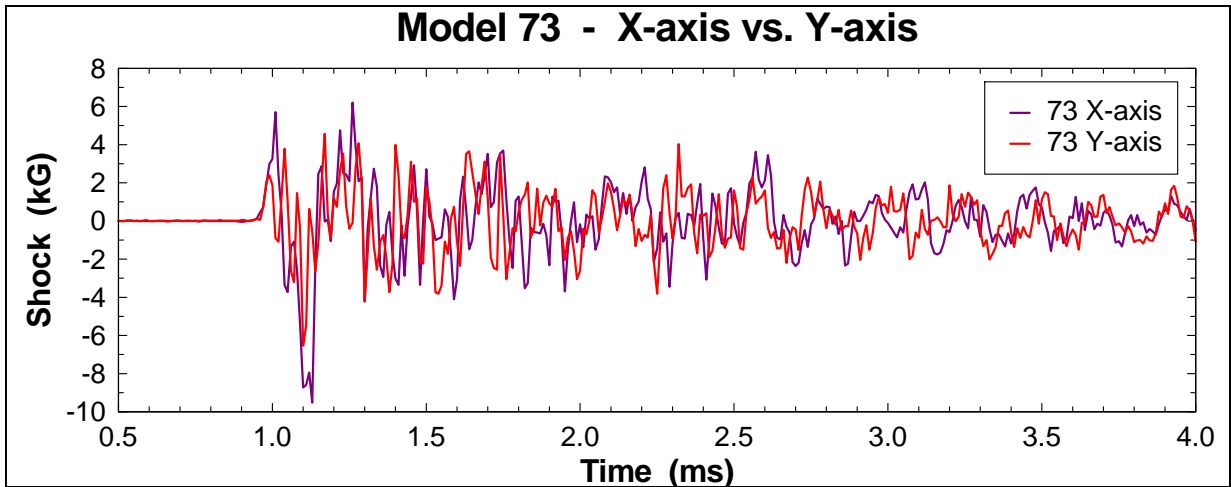
Figure 25. Test 5 of the triaxial accelerometer and Stycast epoxy (x and y axis).
