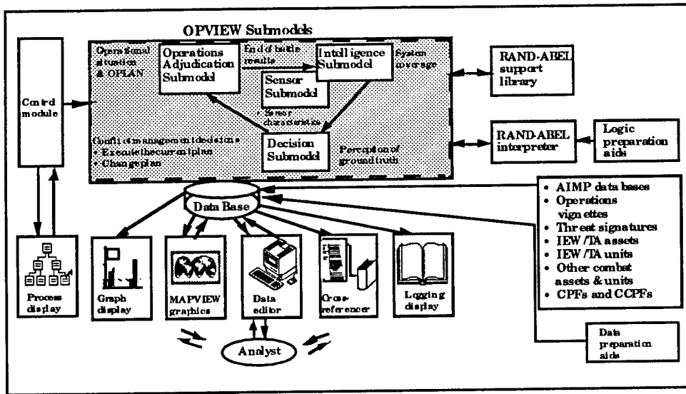
Figure 35—Modeling Environment
