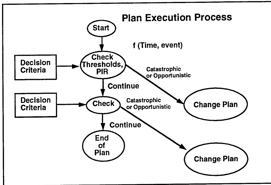
Figure 33—Decision Submodel
