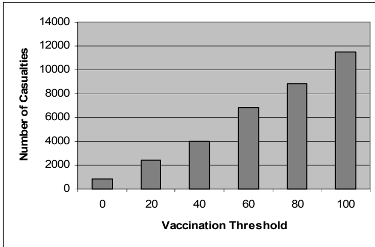
Figure 5: The Effect of Vaccination Threshold – Base Case 1
