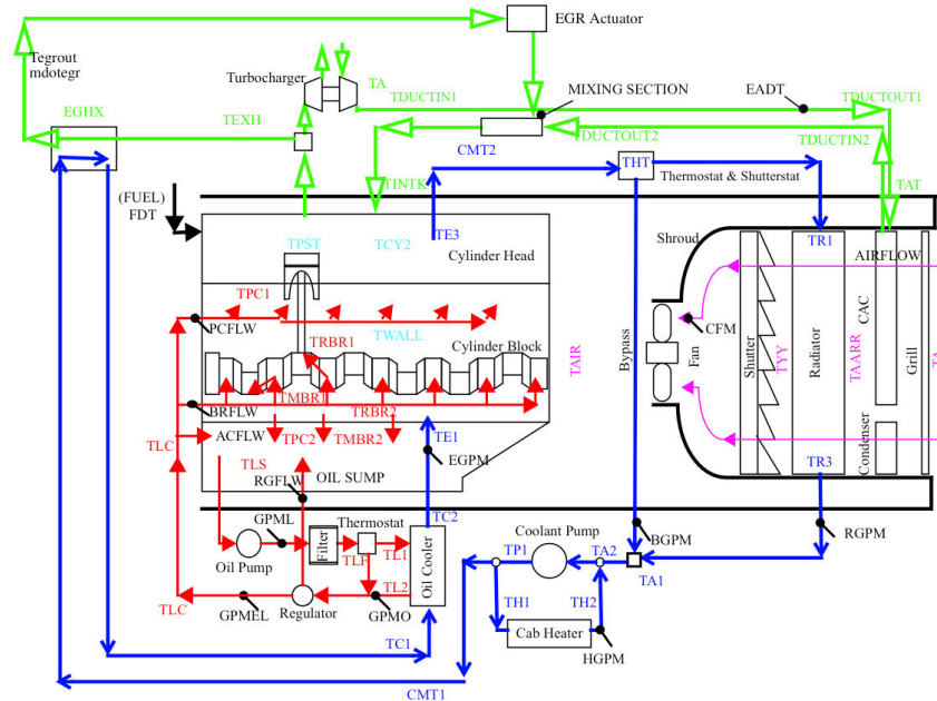
Figure 2.4-2. Uncontrolled EGR cooling system (UCEGRC) schematic.
