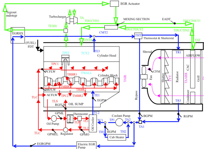
Figure 2.4-3. Controlled EGR cooling system (CEGRC) schematic.
