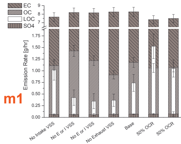
Figure 3-23c. Variation in particle composition at mode 1 operating condition versus different oil consumption engine builds.
