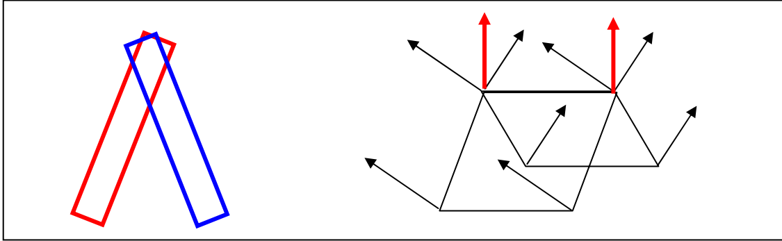
Figure 3. Normal vectors are averaged to represent the surface correctly.
