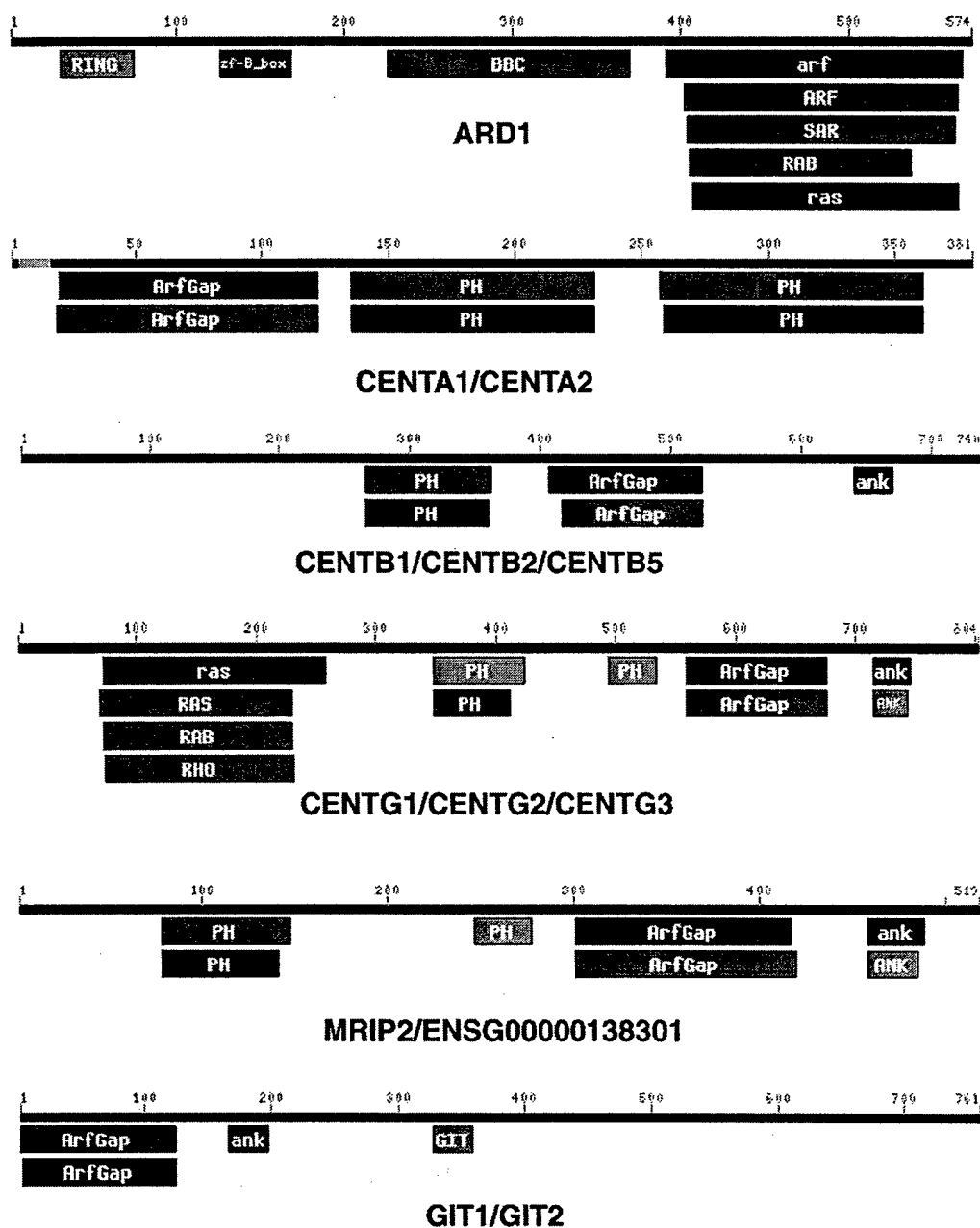
Fig. 4. Domain structure of putative human ArfGAPs. The diagrams were generated by performing a CD computer search, which scans proteins for segments that match domain profile databases [363]. Only domains that match domain profiles are detected. Only one representative structure for each group of related proteins is shown.
