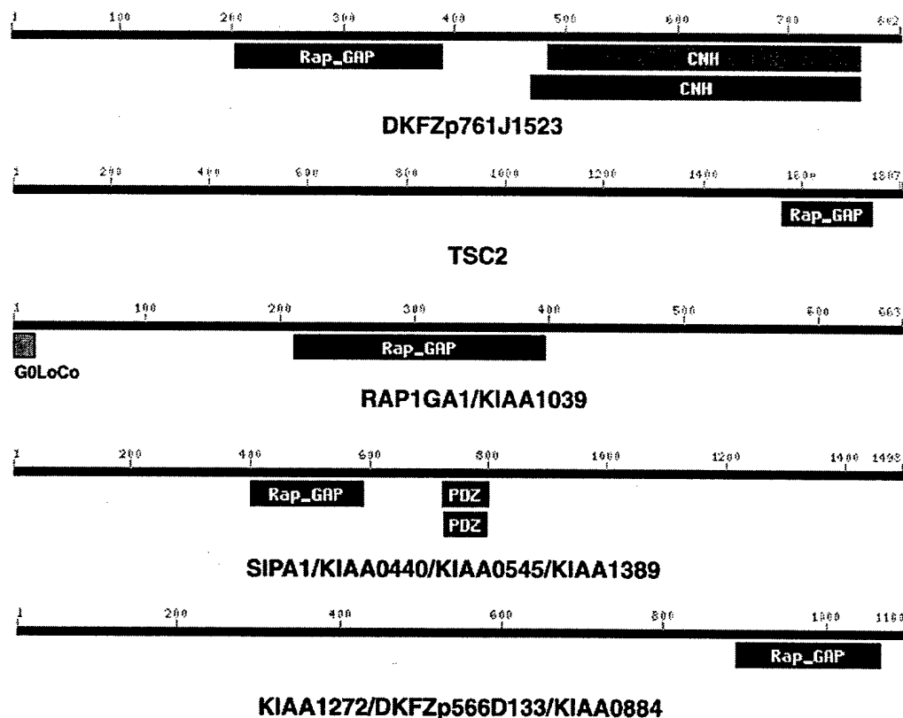
Fig. 8. Schematic structure of human RapGAP domain containing proteins. See Fig. 4 legend for details.
