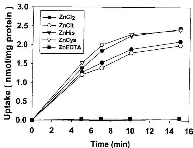
Fig. 1. Time course of ^{65}\text{Zn} uptake from \text{ZnCl}_2 , Zn-Citrate, Zn-Histidine, Zn-Cysteine and Zn-EDTA by VP mitochondria. Substrates contained 20\ \mu\text{M} \text{ZnCl}_2 and 60\ \mu\text{M} ligand. Incubation at 37^\circ\text{C} .
