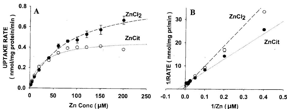
Fig. 9. Zinc uptake from ZnCl 2 and Zn-Citrate in rat liver mitochondria: 15 min incubation at 37 °C.
