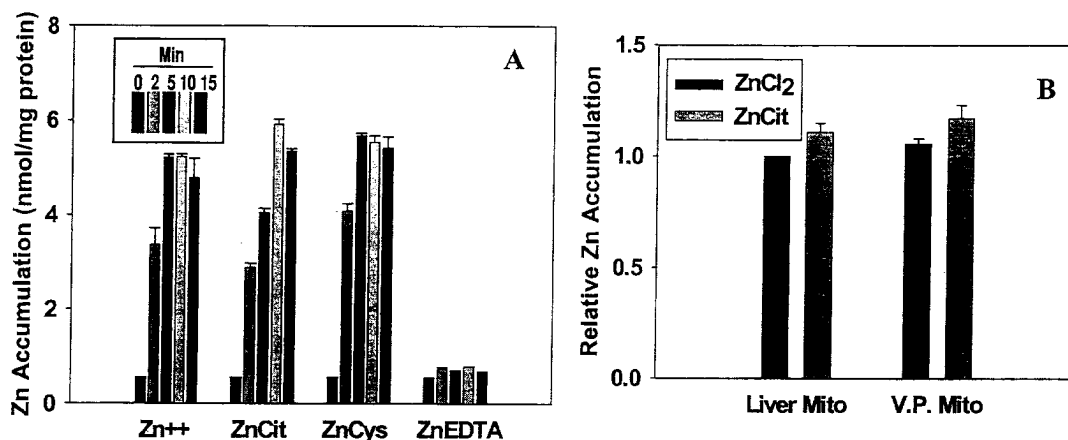
Fig. 10. Total zinc accumulation in mitochondria. Zinc concentration was 30 \mu\text{M} and ligands were 90 \mu\text{M} . After incubation, reaction tubes were rapidly centrifuged and mitochondrial pellets were digested and assayed for total zinc by atomic absorption. (A) Zinc accumulation by liver mitochondria. (B) Comparison of total zinc accumulation in liver and prostate mitochondria.
