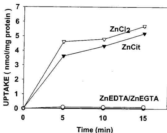
Fig. 8. Time course of 65 Zn uptake from Zn-EDTA, Zn-EGTA, Zn-Citrate and ZnCl 2 by rat liver mitochondria. Substrates contained 50 \mu M ZnCl 2 and 150 \mu M ligand.
