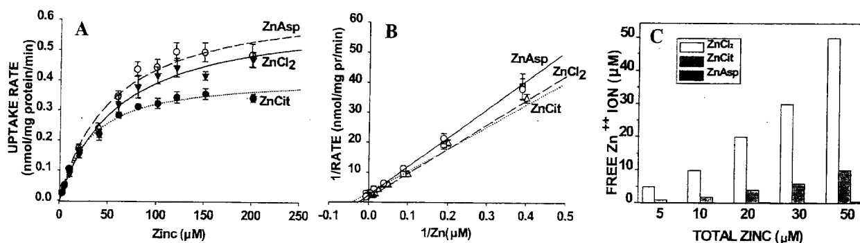
Fig. 2. Zinc uptake from \text{ZnCl}_2 , Zn-Aspartate and Zn-Citrate in rat ventral prostate mitochondria. Uptake was performed at 37^\circ\text{C} , 15 min incubation. For zinc concentrations from 50 to 200\ \mu\text{M} , zinc uptake was linear for about 20–30 min. (A) Hyperbolic plot; (B) Lineweaver–Burk plot; (C) free zinc ion concentration.
