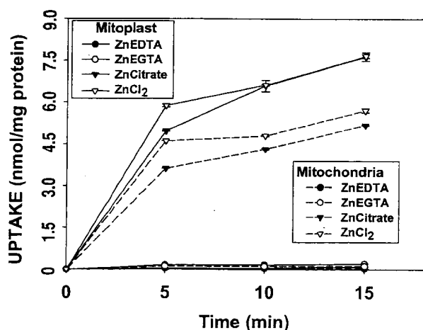
Fig. 11. Time course of zinc uptake from Zn-EDTA, Zn-EGTA, Zn-Citrate and \text{ZnCl}_2 in rat liver mitochondria vs. mitoplasts at 37°C. Substrates contained 50 \mu\text{M} \text{ZnCl}_2 and 150 \mu\text{M} ligand.
