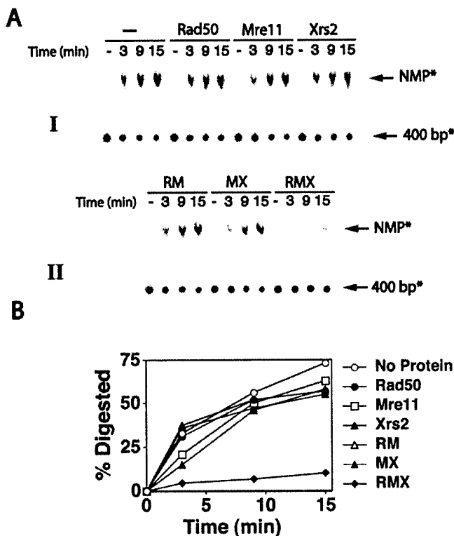
FIG. 8. Xrs2 is needed for protection of DNA ends against \lambda exonuclease digestion. A , the 5' ^{32} P-labeled duplex (9.5 nM DNA ends) was mixed with 60 nM each of Rad50, Mre11, Xrs2, Rad50-Mre11 (RM), Mre11-Xrs2 (MX), and Rad50-Mre11-Xrs2 (RMX), and then \lambda exonuclease was added and the incubation continued at 0 °C. Samples were drawn at the indicated times, deproteinized, and resolved by TLC. B , the data points from phosphorimaging analysis of the TLC plates in A were plotted.
