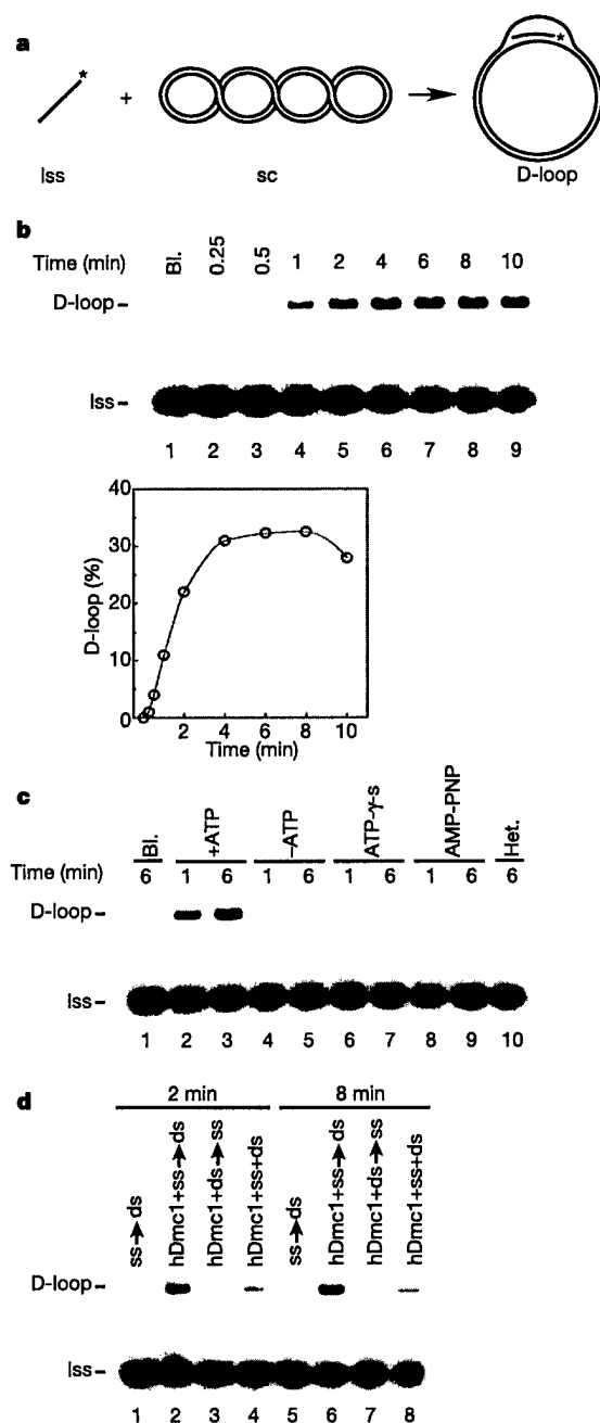
Figure 3 hDmc1 mediates robust D-loop formation. a , Reaction diagram: pairing of OL2 (lss) with pBluescript replicative form I DNA (sc) yields D-loop. b , D-loop formation as a function of time. BI, reaction blank without hDmc1. c , The dependence of D-loop formation on ATP and DNA homology. The heterologous DNA ( \phi X174 replicative form I DNA, designated as Het in lane 10) was used with hDmc1 and ATP. BI, reaction blank with the homologous DNA substrates but no hDmc1. d , The level of D-loop was examined as a function of the order of addition of reaction components.
