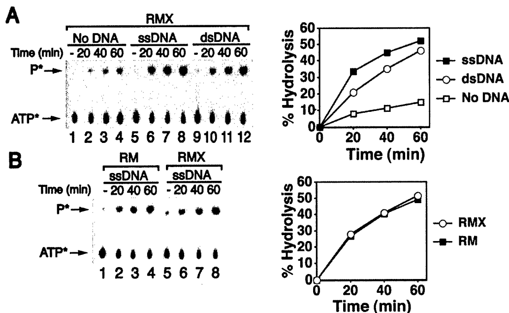
FIG. 6. Effects of Mre11 and Xrs2 on the Rad50 ATPase activity. A, the Rad50-Mre11-Xrs2 (RMX) complex (1.4 \mu M) was incubated with [ \gamma - 32 P]ATP (150 \mu M) at 30 °C without DNA and with \phi X174 (+) strand (ssDNA; 23 \mu M nucleotides) or linear duplex (dsDNA; 23 \mu M bp). Samples were drawn at the indicated times, deproteinized, and then analyzed by TLC. The data points from phosphorimaging analysis of the TLC plates were plotted. B, the Rad50-Mre11 (RM) and RMX complexes (1.2 \mu M each) were incubated at 30 °C with 150 \mu M [ \gamma - 32 P]ATP with ssDNA. Samples were drawn at the indicated times, deproteinized, and then analyzed by TLC. The data points from phosphorimaging analysis of the TLC plates were plotted.
