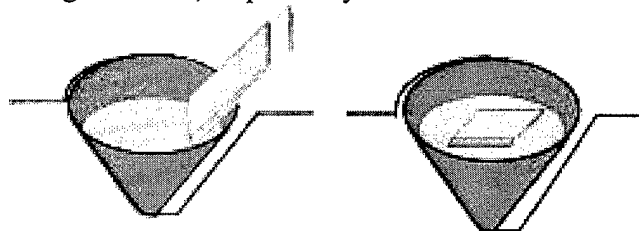
Figure 4. Schematics of experiment with bulk pool of gallium melt using an alumina coated conical heater assembly.
