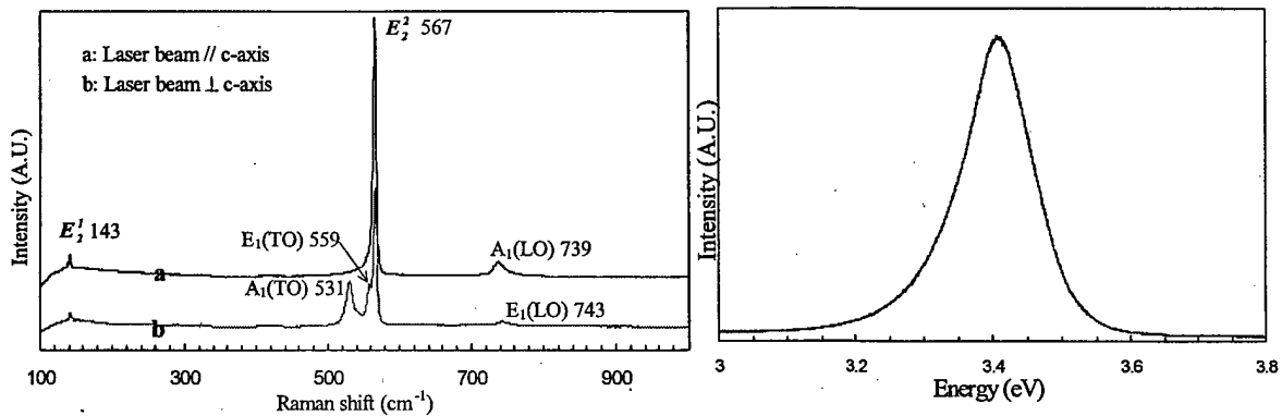
Figure 41. Raman spectrum obtained using back-scattered configuration for one of the resulting GaN films.
