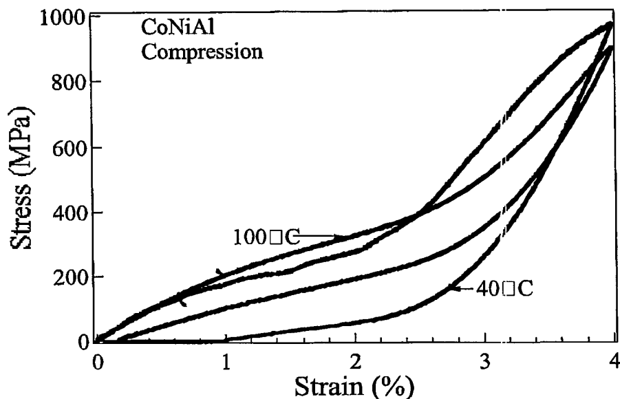
Figure 2 The pseudoelastic response of a stabilized specimen at 40°C (third cycle) and 100°C (fifth cycle). The recoverable strain (including elastic recovery) is as high as 4% at 100°C.
