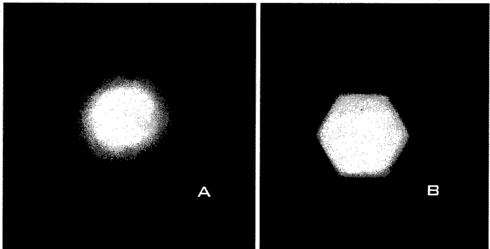
Figure 4. Light profiles from the 10 LEDs for DEMO 1 with the LSD (A) and the LHS (B) in the light path.
