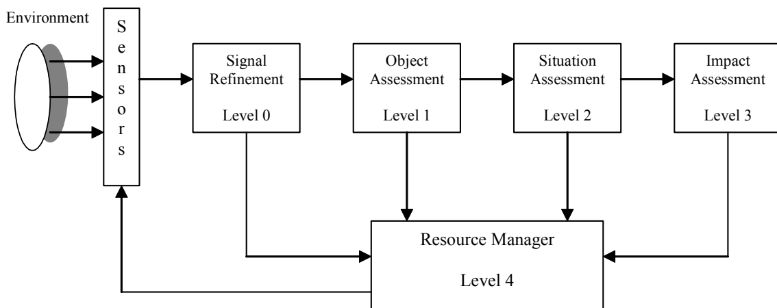
Figure 1: JDL Model.
