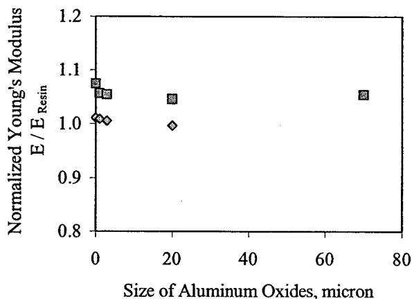
Figure 4 Effect of Particle Size on Young's Modulus with 1 vol. % (3.6 wt. %: 50 nm, 3.7 wt. %: 3-70 \mu m) and 3 vol. % (10.8 wt. %: 50 nm, 11.2 wt. %: 3-70 \mu m) Aluminum Oxides. (Square and diamond symbols indicate normalized Young's modulus with 3 vol. % and 1 vol. % particle loadings, respectively.)
