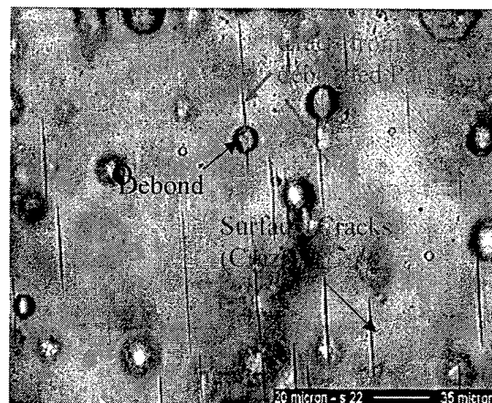
Figure 7 Observed failure modes in composite with 3 vol. % of 20 μm aluminum oxide particles
