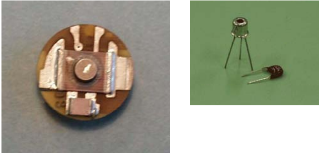
Figure 4 State of the art detonator (left) and mock-up of MEMS EFI (right) on the same scale.
