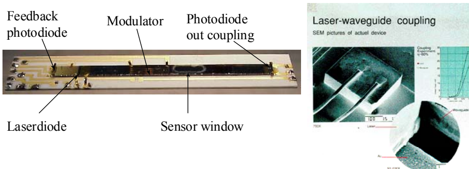
Figure 1 Mach-Zehnder sensor (left) and its laser waveguide coupling (right)
