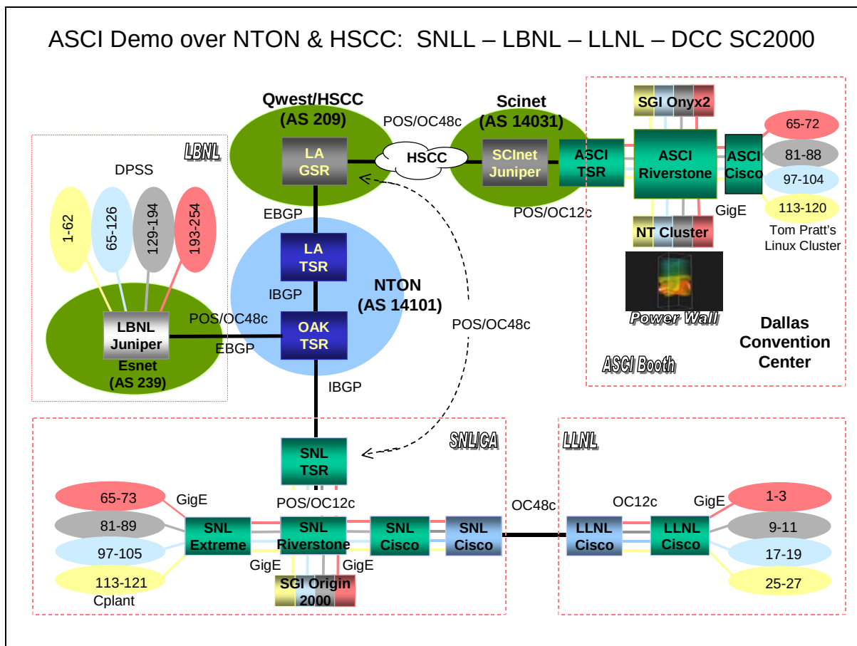
Figure 4-6. NTON Configuration in support of ASCI Demo at SC2000.
