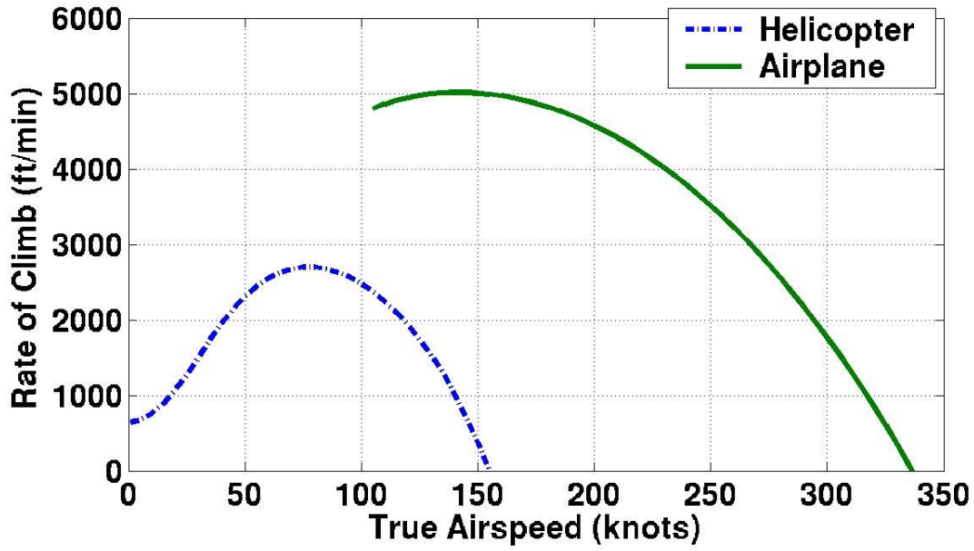
Figure 64: MTR rate of climb capability versus airspeed at mean sea level conditions for both flight modes.
