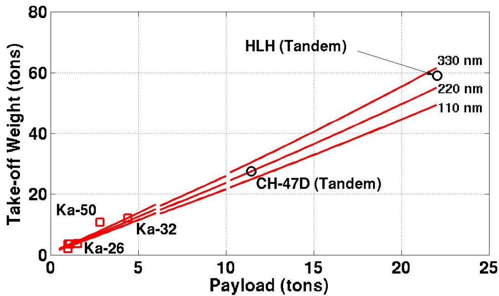
Figure 21: Predicted gross takeoff weight versus payload for coaxial dual rotor helicopters.
