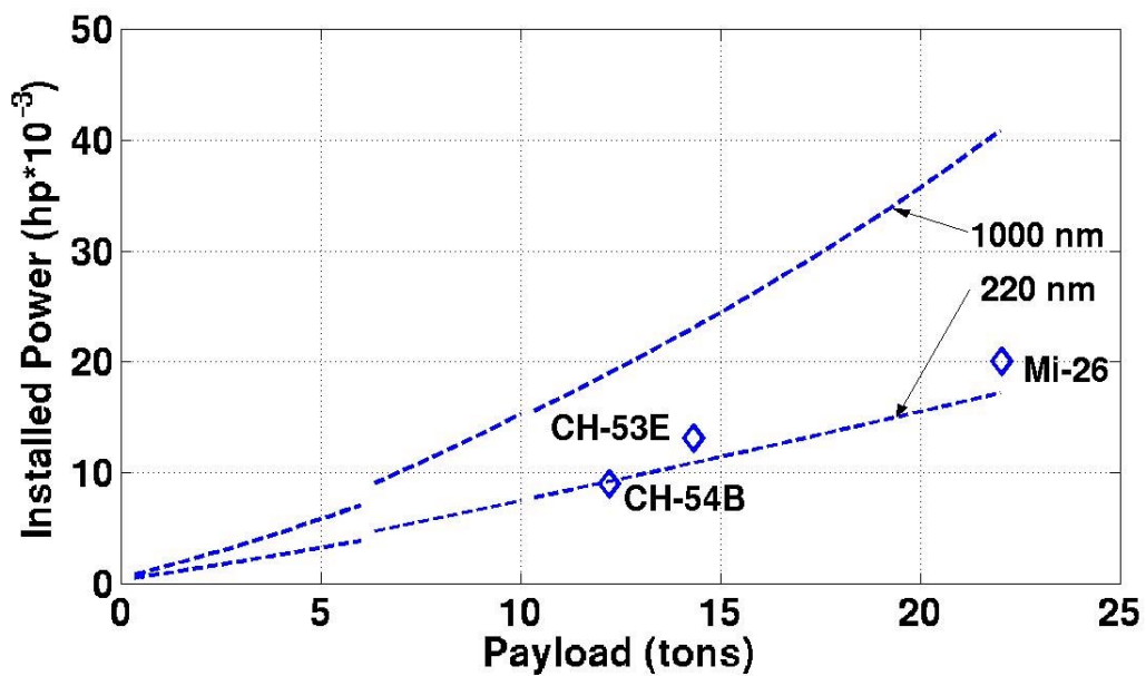
Figure 32: Predicted power requirements versus payload for a single rotor helicopter with ranges of 220 nm and 1,000 nm.
