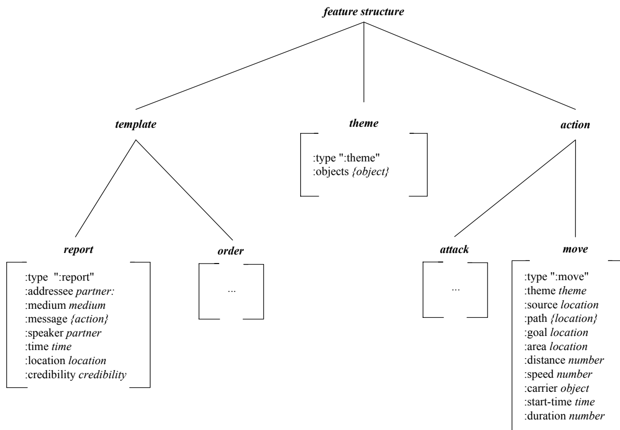
Figure 2: A Part of the Feature Structure Hierarchy.
