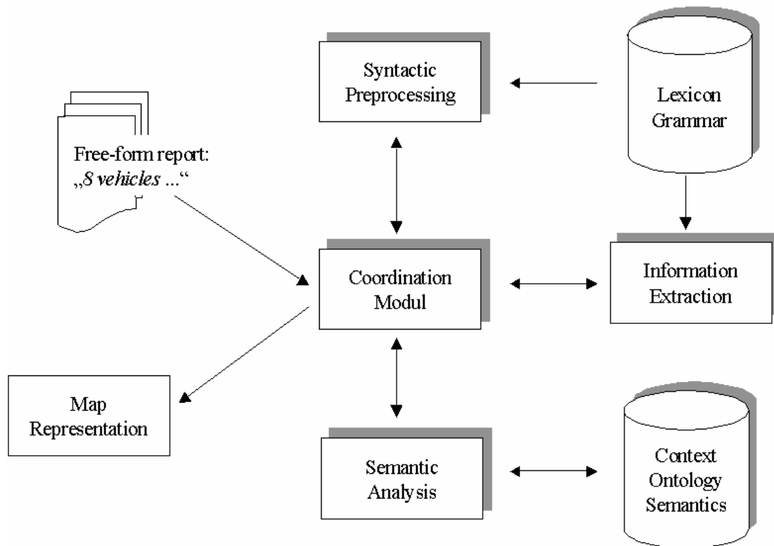
Figure 1: The Architecture of SOKRATES.
