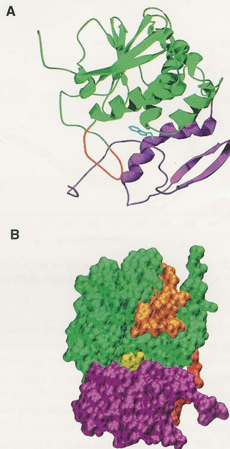
Figure 1. rRTA structure. (A) The N-terminal domain is shown in green, loop (amino acids 34–43) in red; C-terminal domain (amino acids 199–267), in purple; and the single tryptophan (amino acids 211), in cyan (1rtc.pdb; Mlsna et al. 1993). (B) Surface model of the opposite side of the molecule. Active site residues E177 and R180 are shown in yellow, and a neutralizing epitope (amino acids 95–110) in orange. Figures drawn with PyMol (Delano Scientific).
