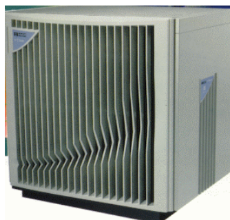
Shared-Memory Servers
