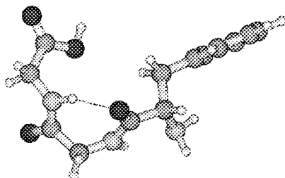
Calculated structure of phe-gly-gly
