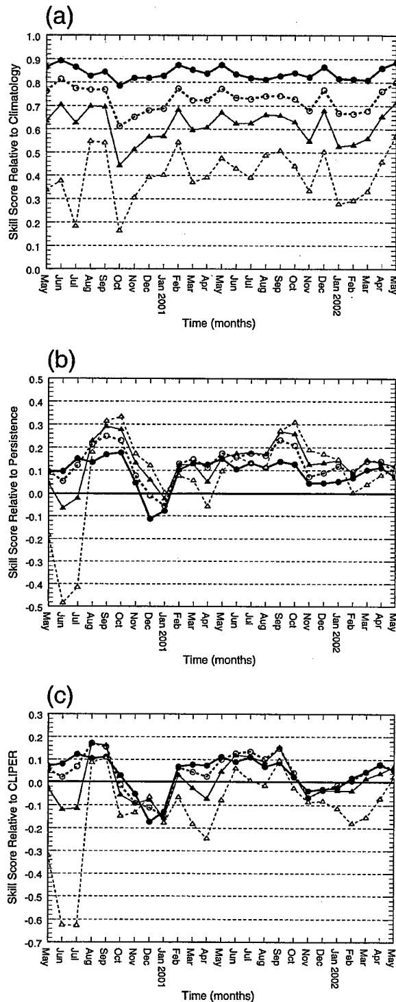
FIG. 3. Skill scores relative to (a) climatology, (b) persistence, and (c) CLIPER for the period May 2000–May 2002 based on a \pm 5\% cutoff value. The bold solid and dashed lines with circles denote the 24- and 48-h skill scores, respectively. The solid and dashed lines with triangles denote the 72- and 120-h skill scores, respectively. The 95% confidence limits are roughly equal to the size of the dots.
