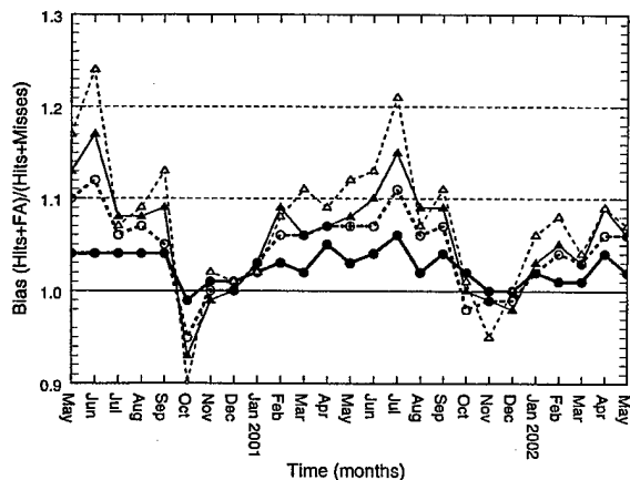
FIG. 11. Forecast bias at 24 (bold line with solid circles), 48 (bold dashed line with open circles), 72 (line with solid triangles), and 120 h (dashed line with open triangles).
