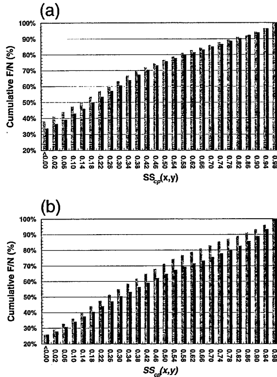
FIG. 6. Cumulative frequency of occurrence normalized by the total number of points ( N ) vs the skill score relative to CLIPER for (a) Dec 2000/2001 and (b) May 2001/2002. Both Dec 2000 and May 2001 are shown in gray; Dec 2001 and May 2002 are shown in black. With the exception of the first bin, the bins are 0.04 wide and the listed abscissa values denote the centers of the bins. All skill scores < 0 are included in the first bin.
