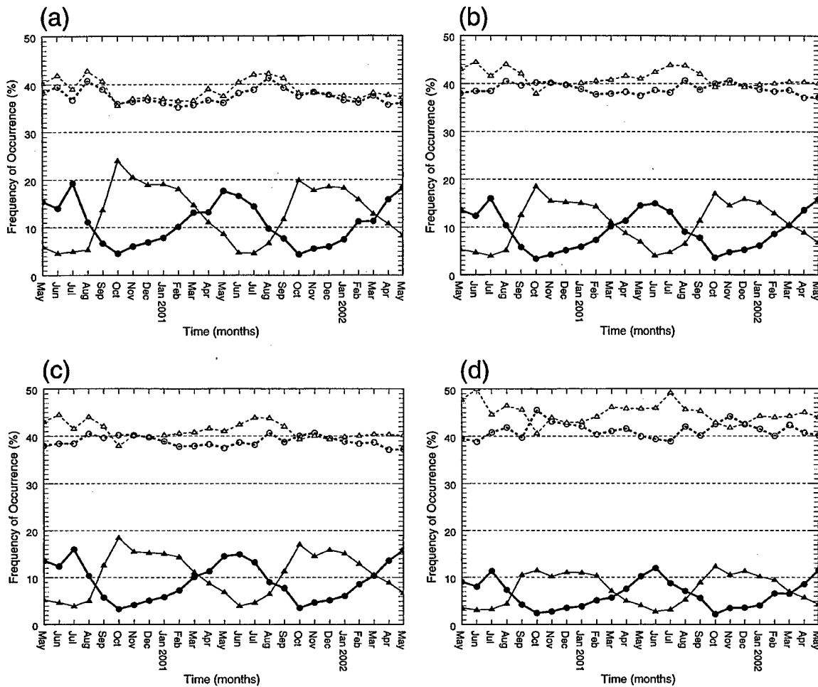
FIG. 9. Threat indexes for a forecasted >5% decrease in sea ice concentration at (a) 24-, (b) 48-, (c) 72-, and (d) 120-h lags. Hits are denoted by a bold line with solid circles, correct rejections by a line with solid triangles, misses by a bold dashed line with open circles, and false alarms by a dashed line with open triangles.
