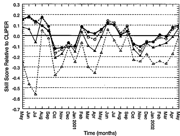
FIG. 8. Skill scores relative to CLIPER for the period May 2000–May 2002 based on a \pm 15\% cutoff value. The bold solid and dashed lines with circles denote the 24- and 48-h skill scores, respectively. The solid and dashed lines with triangles denote the 72- and 120-h skill scores, respectively.
