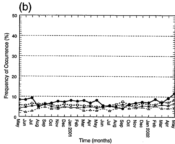
FIG. 12. (a) Threat indexes for forecasted melt of sea ice at 24-h lag. Hits are denoted by a bold line and solid circles, correct rejections by a line and solid triangles, misses by a bold dashed line with open circles, and false alarms by a thin line with open triangles. (b) Total correct forecasts at 24 (bold line with solid circles), 48 (bold dashed line with open circles), 72 (line with solid triangles), and 120 h (dashed line with open triangles).
