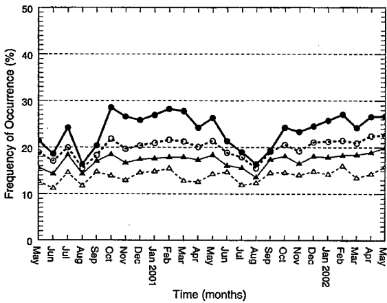
FIG. 10. Total correct (hits + correct rejections) forecasts at 24 (bold line with solid circles), 48 (bold dashed line with open circles), 72 (line with solid triangles), and 120 h (dashed line with open triangles).
