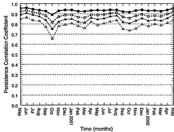
FIG. 4. Persistent correlation coefficient for the period May 2000–May 2002 based on a \pm 5\% cutoff value. The bold solid and dashed lines with circles denote the 24- and 48-h skill scores, respectively. The solid and dashed lines with triangles denote the 72- and 120-h skill scores, respectively. The 95% confidence limits are roughly equal to the size of the dots.
