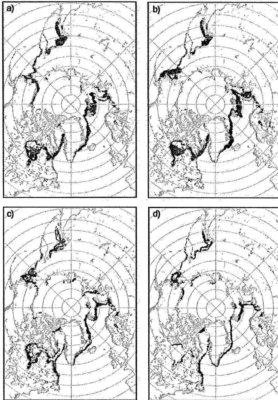
FIG. 7. Spatial distributions of SS_g for (a) Dec 2000, (b) Dec 2001, (c) May 2001, and (d) May 2002. Skillful forecasts ( SS_g > 0.1 ) are denoted by blue and nonskillful forecasts ( SS_g < 0.1 ) are denoted by red. Regions with unchanged sea ice or ocean conditions are denoted by white.
