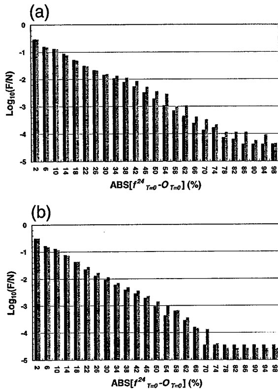
FIG. 5. Logarithmic frequency of occurrence normalized by the total number of points ( N ) vs the absolute difference between the 24-h forecast and observed values for (a) Dec 2000/2001 and (b) May 2001/2002. Both Dec 2000 and May 2001 are shown in gray; Dec 2001 and May 2002 are shown in black. The bins are 4% wide and the listed abscissa values denote the centers of the bins.
