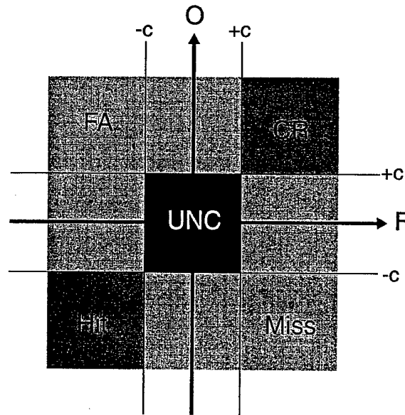
FIG. 2. Contingency diagram for threat indexes: F and O represent the forecast and observed values, respectively; hit, miss, FA, CR, and UNC represent hits, misses, false alarms, correct rejections, and unchanged, respectively. All are defined in the text. Here, \pm c represents the positive and negative cutoff values ( \pm 5\% or \pm 15\% ) used in this study.
