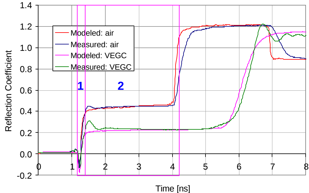
TDR to Uniform Fillings: Air and VEGC
