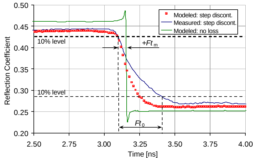
TDR Waveforms Effected by Step Discontinuity
