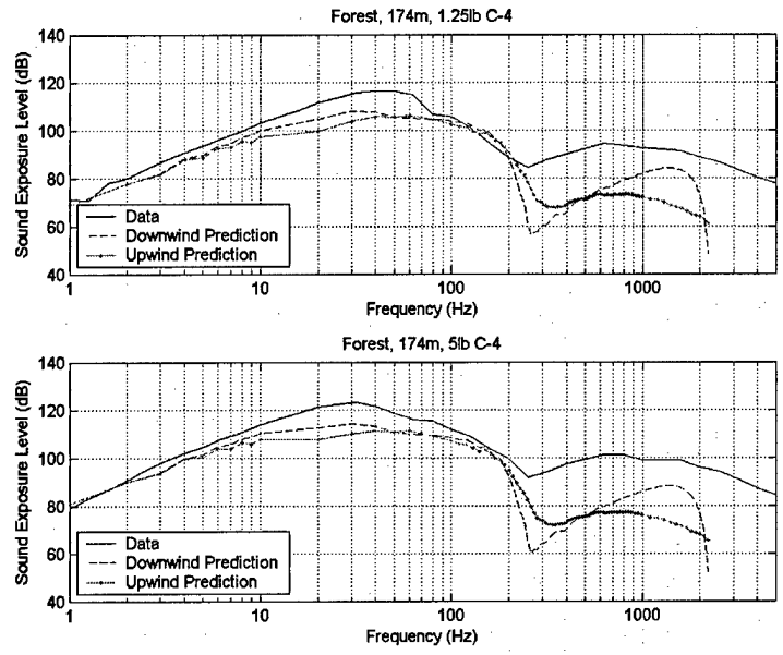
Figure 12: Comparison of forest measurements to GFPE model, 174 m.
