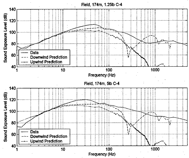
Figure 13: Comparison of open field measurements with GFPE model, 174 m.
