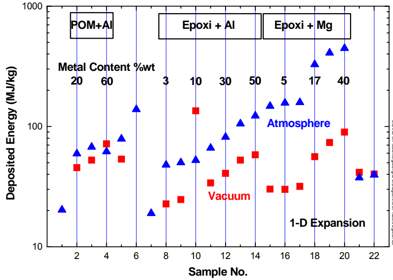
Diagram 24 Comparison of the deposited energy
