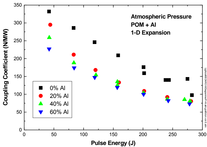
Diagram 6 Coupling Coefficient vs. pulse energy
