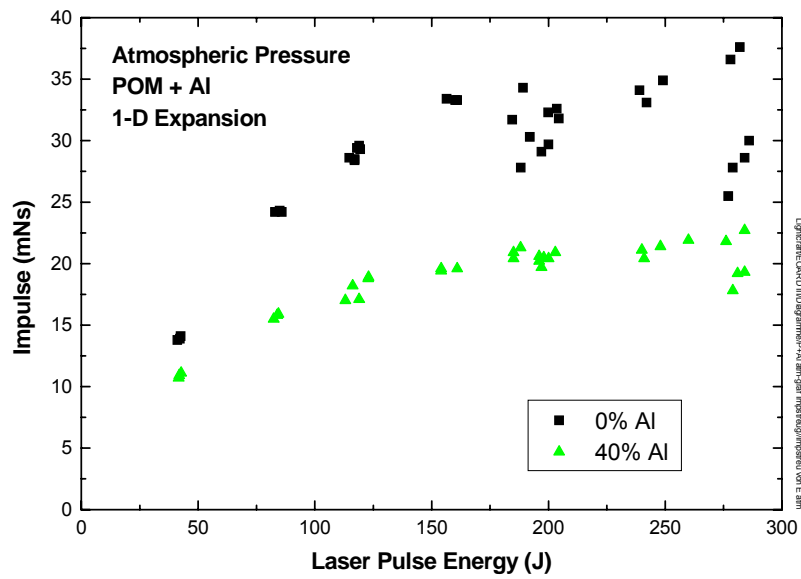
Diagram 5 Impulse data scatter of individual shots vs. pulse energy
