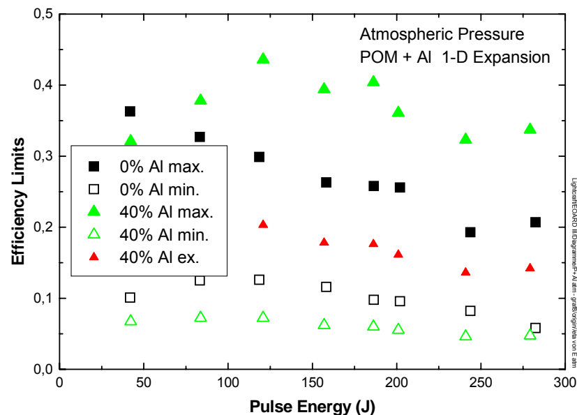
Diagram 8 Limiting values of the jet efficiency vs. pulse energy
