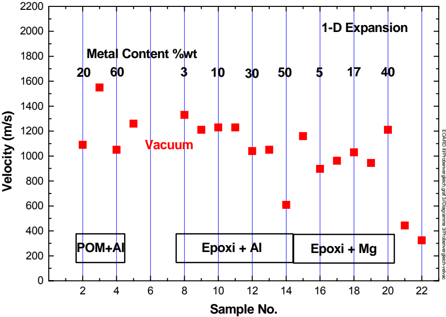
Diagram 26 Comparison of the jet velocity
