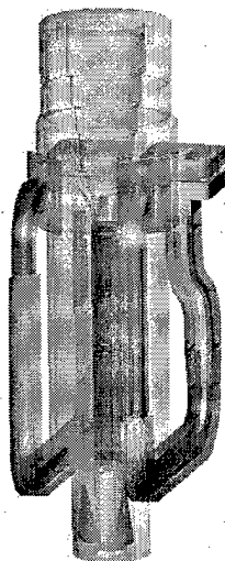
Fig. 4. Input coupler design details.
