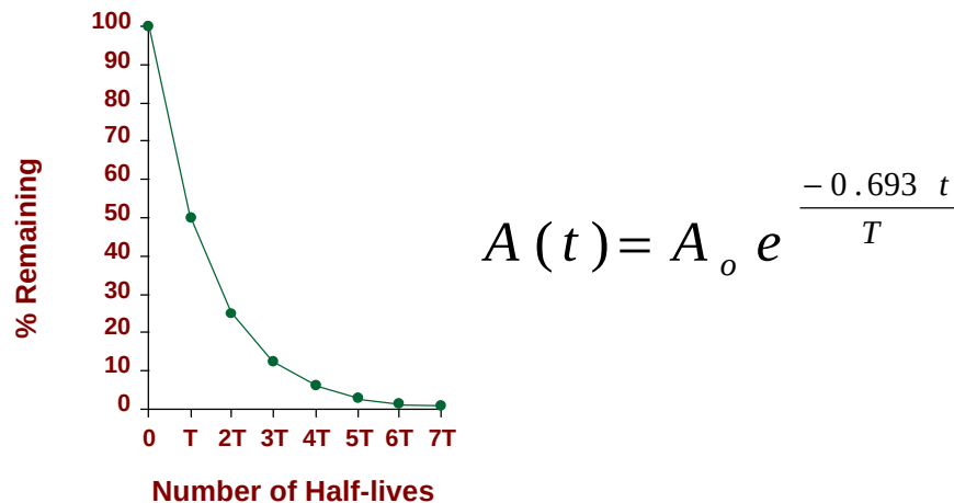
Figure 3-F: The Transformation of a Radionuclide over time
