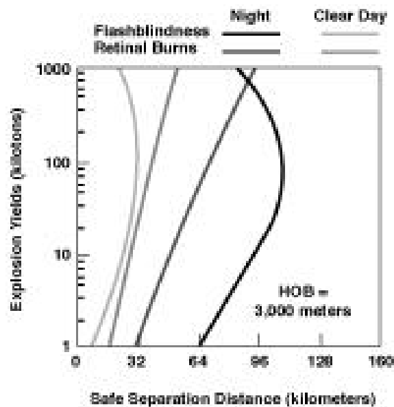
Figure 2-E: Flashblindness and Retinal Burn Safe Separation
