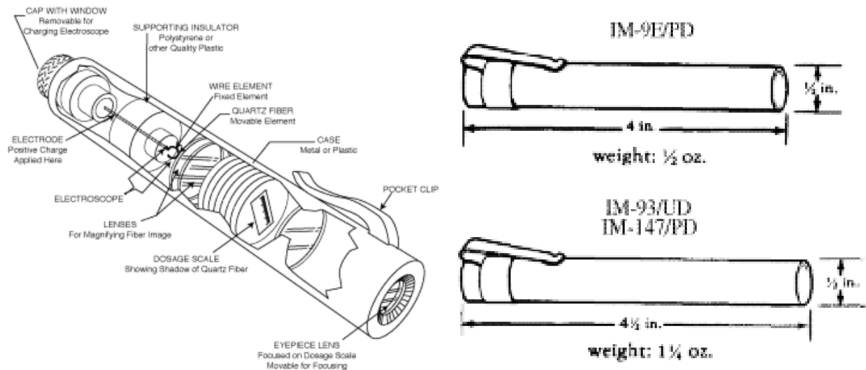
Figure 7-A: Army Pocket Dosimeter
