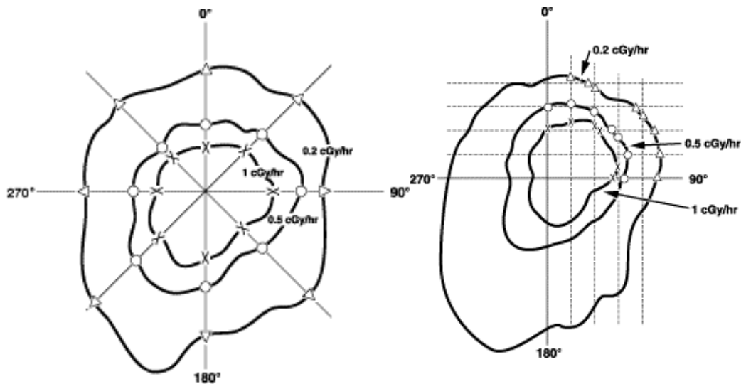
Figure 3-E: Radiation Survey Techniques. Radial Plot (left) and Grid Plot (right)
