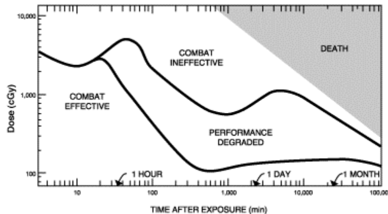
Figure 2-B: Expected Response to Radiation for Physically Demanding Tasks
