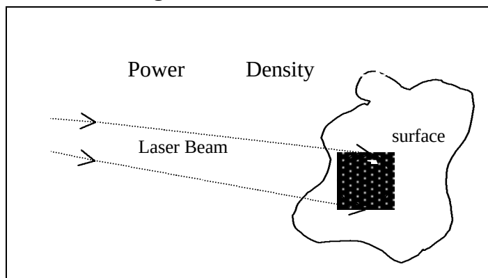
Figure 6-C: Irradiance
