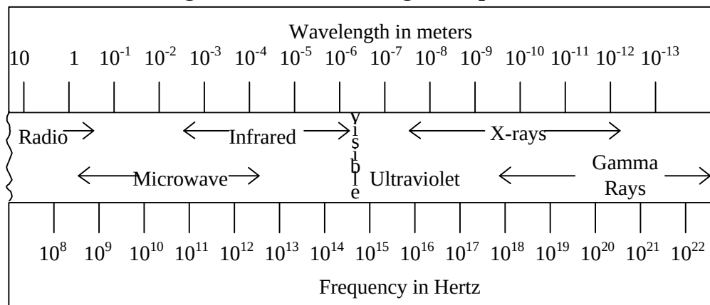
Figure 6-B: Electromagnetic Spectrum
