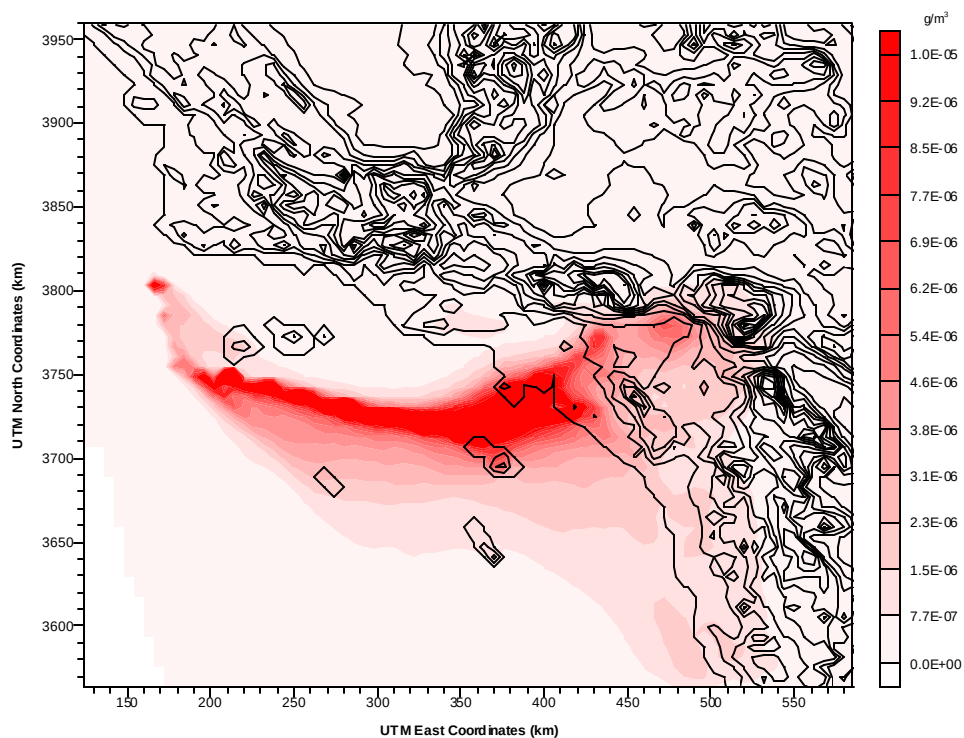
Figure 2-10. Simulated NO x Concentration Time Average, Proposed Shipping Lane, 2-6 September 1997
