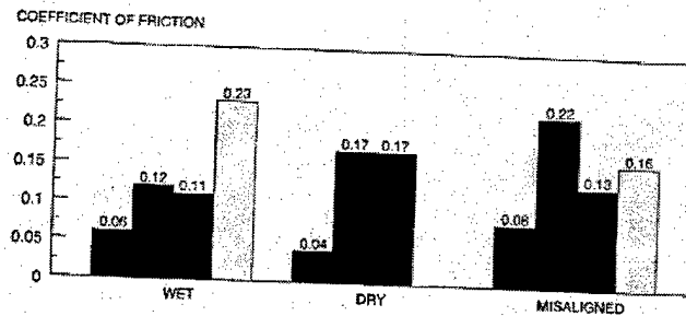
FEROFORM T814 PERFORMANCE-STATIC FRICTION
