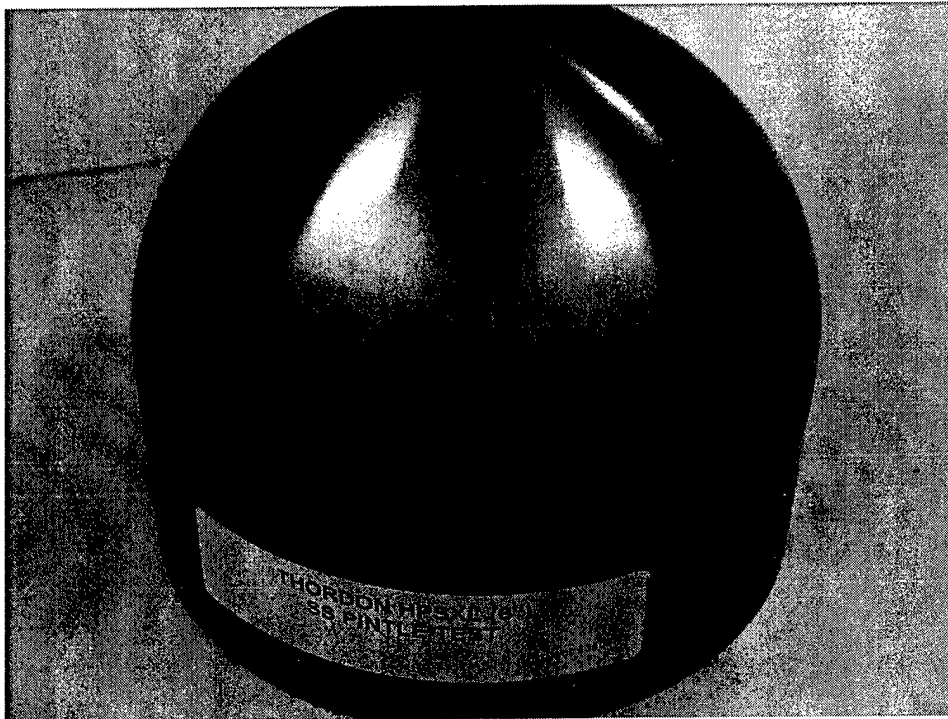
Figure B7. Overview of Thordon HPSXL 6" pintle. Note staining of pintle on loaded side.
