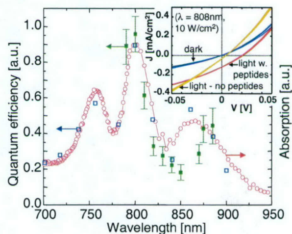
Fig. 18. The photocurrent spectrum of solid-state photovoltaic devices employing bacterial reaction centers (RCs). A comparison between the photocurrent spectrum of solid-state (■) and wet electrochemical cell devices (□), and the solution absorption spectrum of the bacterial reaction centers (—○—), demonstrates that the observed photocurrent originates in the RCs. Inset: stabilization of RC complexes with A 6 K/V 6 D peptides improves the internal quantum efficiency of the devices to 12% under short circuit conditions.
