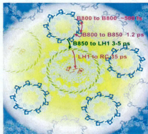
Photosynthetic Machinery of purple bacteria
