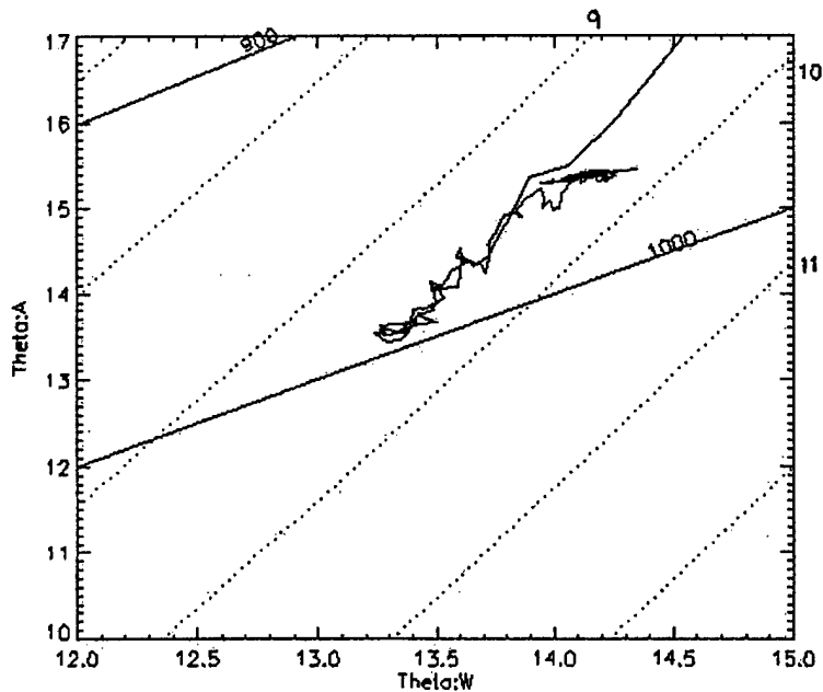
Figure 15. Same as Figure 13 but for RF01/PF04. The data points in the cooled absolute potential temperature region are aligned along a constant total mixing ratio line (dotted lines) indicate that radiative cooling is the main cause of the cooling.
