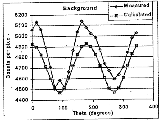
Fig. 8. Measured and calculated values of n_b + n_s near one of the lesions in the cylindrical phantom. Views were obtained over 345^\circ , with 15^\circ between views. The minimum LCD, at \theta = 0^\circ , was 3.85 cm, and the maximum LCD, at \theta = 180^\circ , was 9.15 cm.
