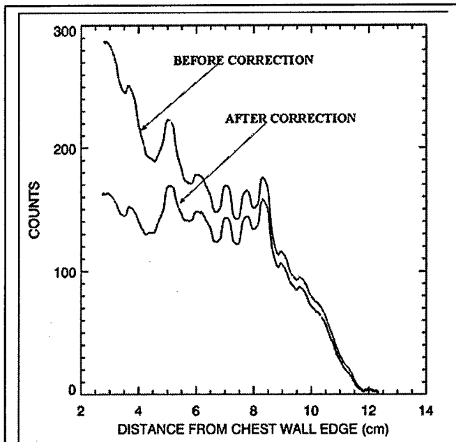
Fig. 10. Profile (single row of pixels) running in the chest wall to anterior direction, and located at the breast midline. Profiles are shown before and after scatter counts have been removed. The region of the image corresponding to the portion of the breast with uniform thickness is seen to have more uniform pixel count following scatter correction.
