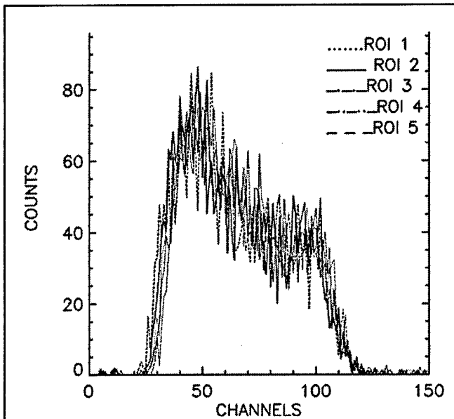
Fig. 7: Composite of 5 spectra taken from 5 ROIs arranged along a line in the medial-lateral direction. Channel 100 corresponds to 140 keV.
