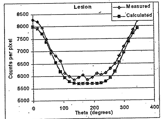
Fig. 9. Measured and calculated values of n_L + n_s for one of the lesions in the cylindrical phantom. Views were obtained over 345^\circ , with 15^\circ between views. The minimum LCD, at \theta = 0^\circ , was 3.85 cm, and the maximum LCD, at \theta = 180^\circ , was 9.15 cm.
