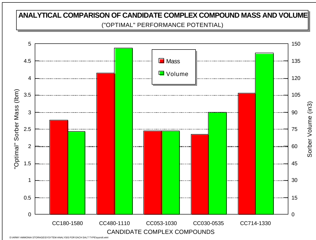
Figure 4. Comparison of Mass and Volume Requirements for Five Candidate Complex Compounds
